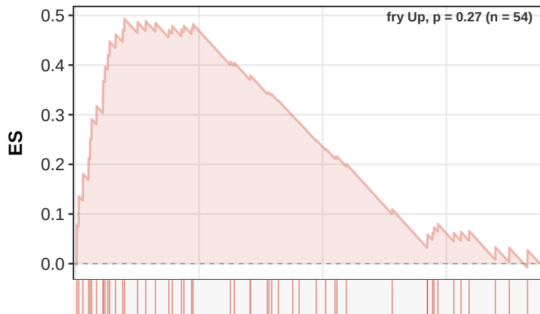
HR-up DEPs -> LR rank
