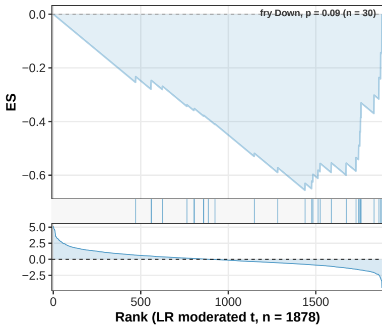
HR-down DEPs -> LR rank
