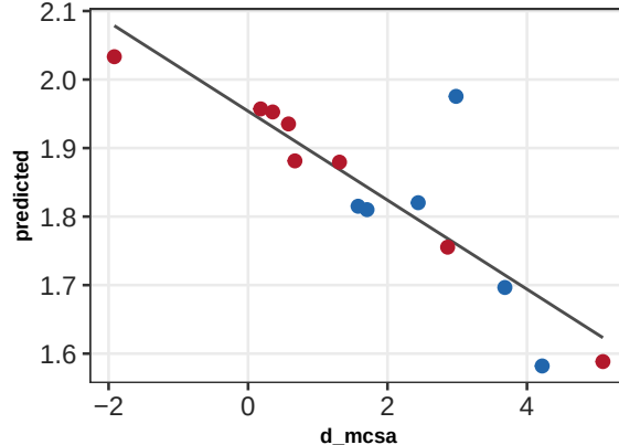
trajectory | spls Q2=0.49 p=0.010
