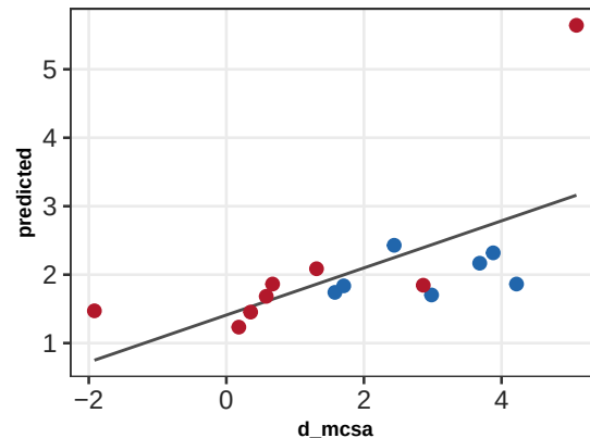
acute | lasso Q2=0.55 p=0.015
