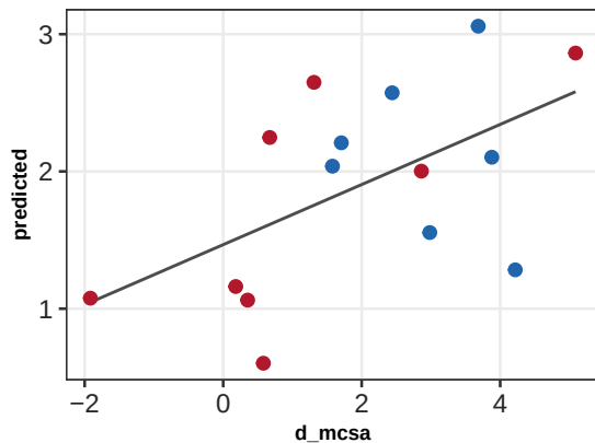
T2 | rf Q2=0.28 p=0.010
