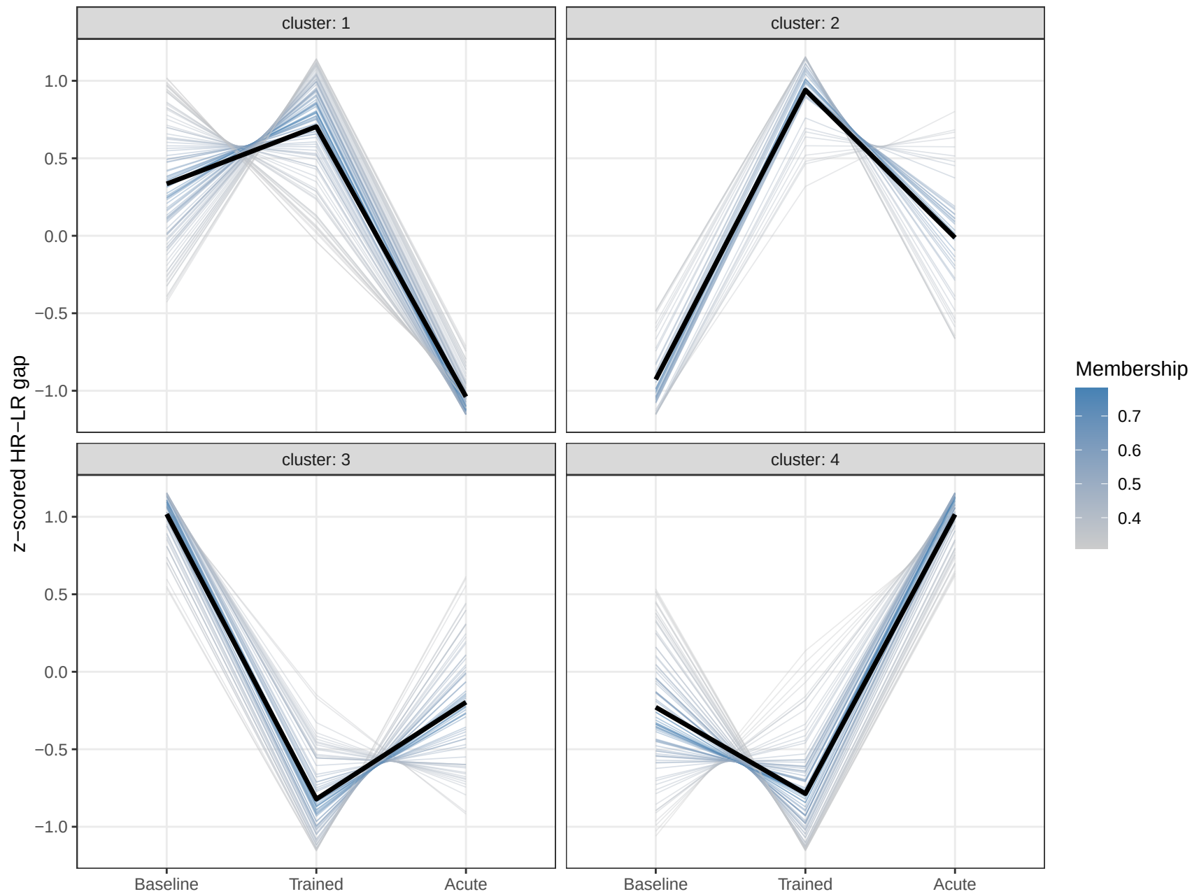
Fuzzy c-means gap-trajectory clusters (z-scored HR-LR gap)
