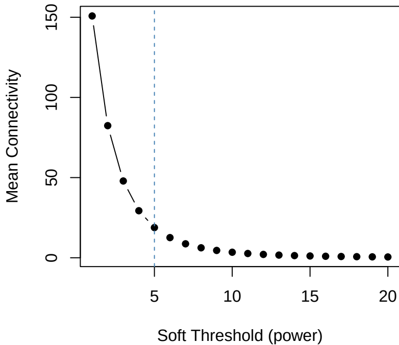
Mean connectivity
