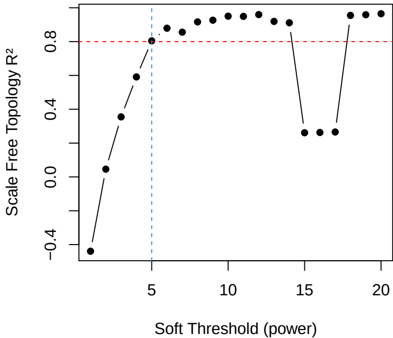
Scale-free fit
