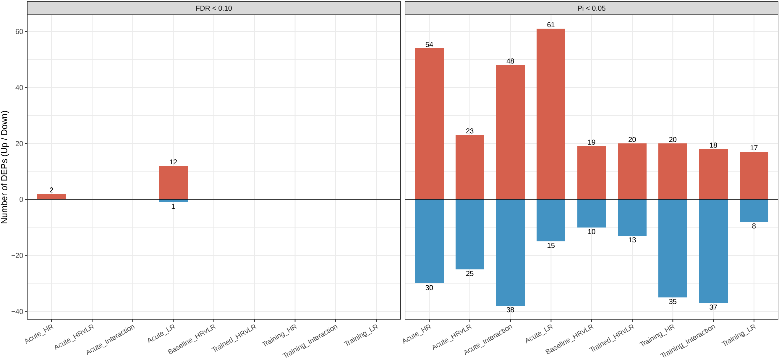
DEP Counts by Significance Criterion
