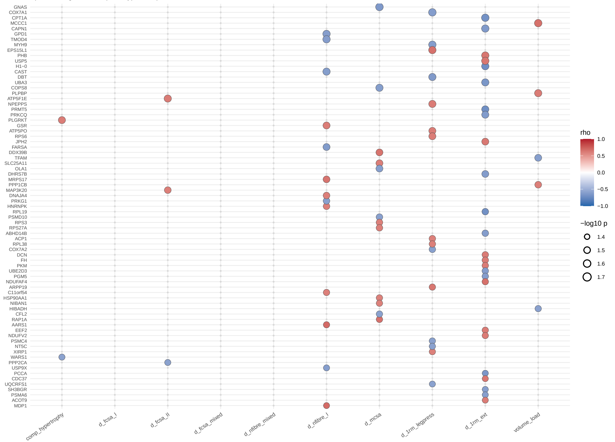
Protein association hits, training change (T2 – T1) (4/7) Spearman against each phenotype; 453 proteins nominal in at least one column; rows 226–300
