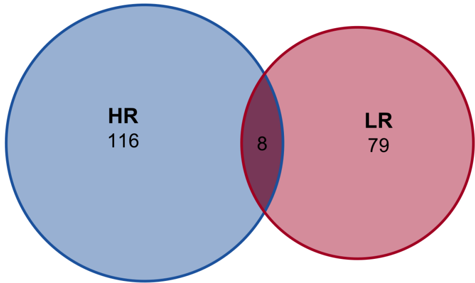
Training Response (T2 - T1, p < 0.0
