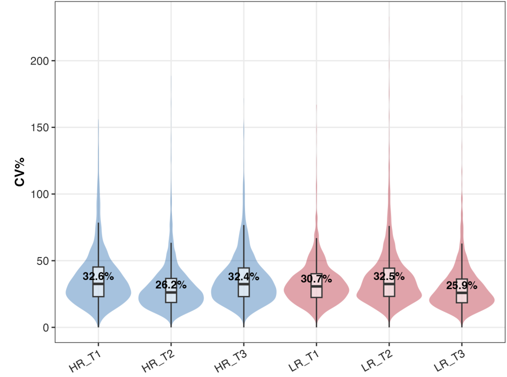
C Inter-Individual Variability CV% per protein (linear scale)
