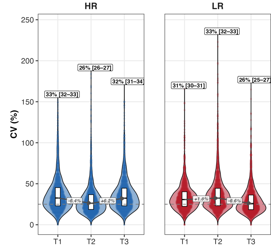
D Inter-Individual Variability (CV%) 1,885 proteins | CV 30% [30–30] training (T1→T2) HR -6.4%, LR +1.8% | acute (T2→T3) HR +6.2%
