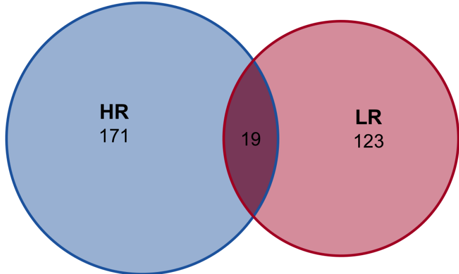
Acute Response (T3 - T2, p < 0.05
