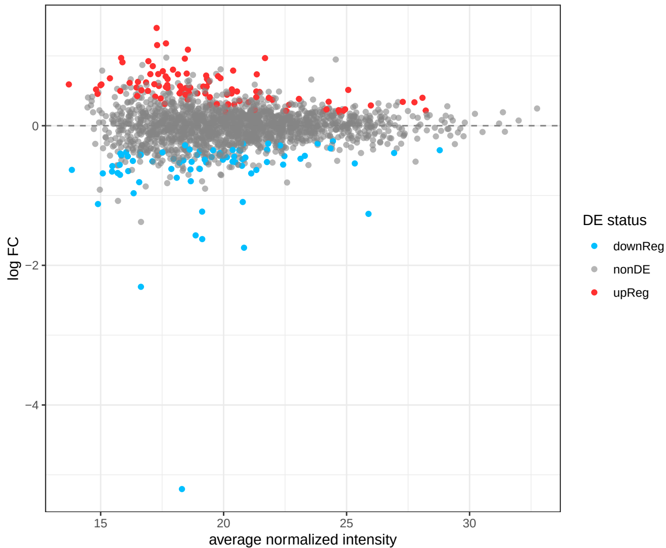
Training_LR, raw p-value
