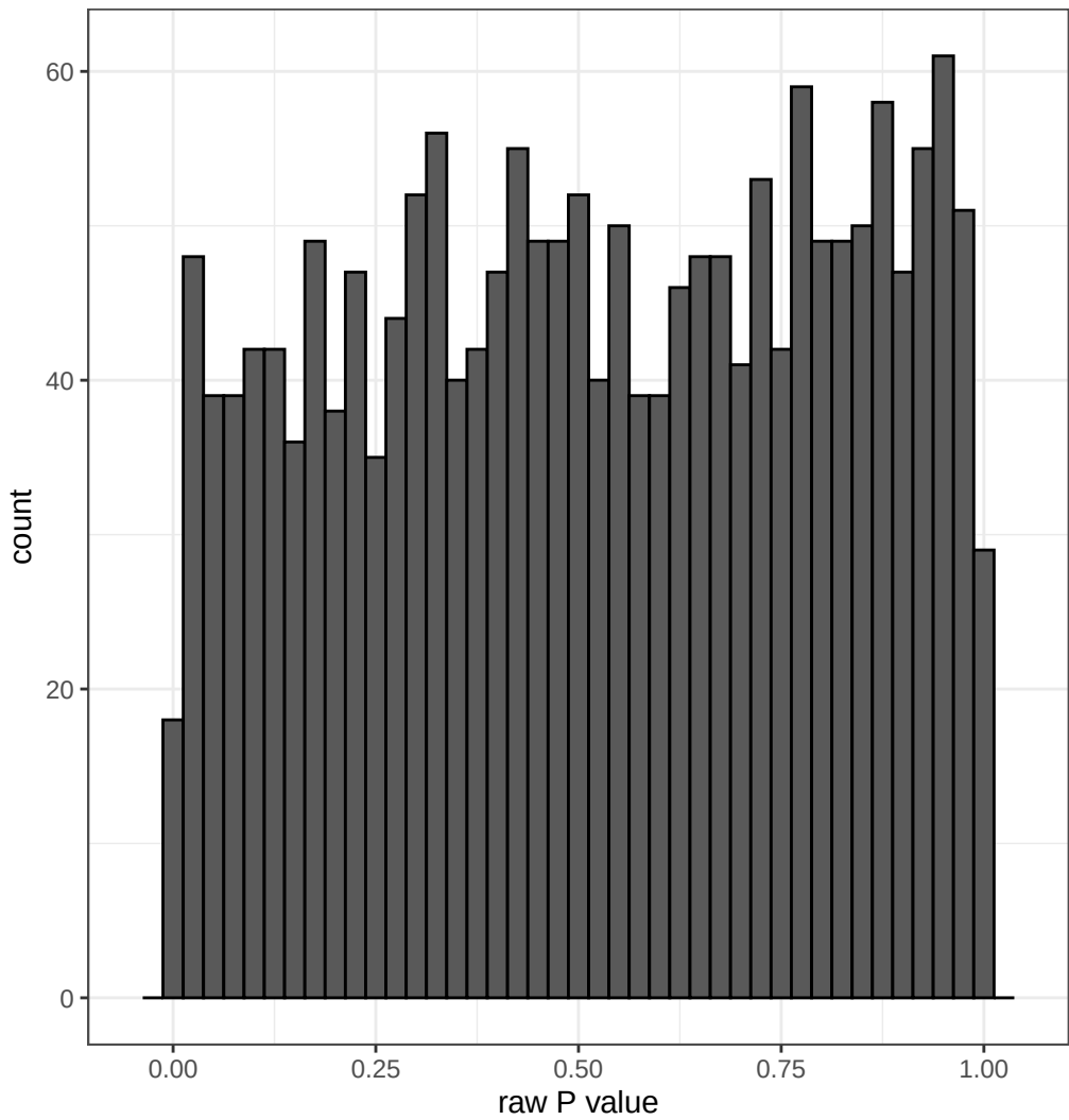
Training_LR
