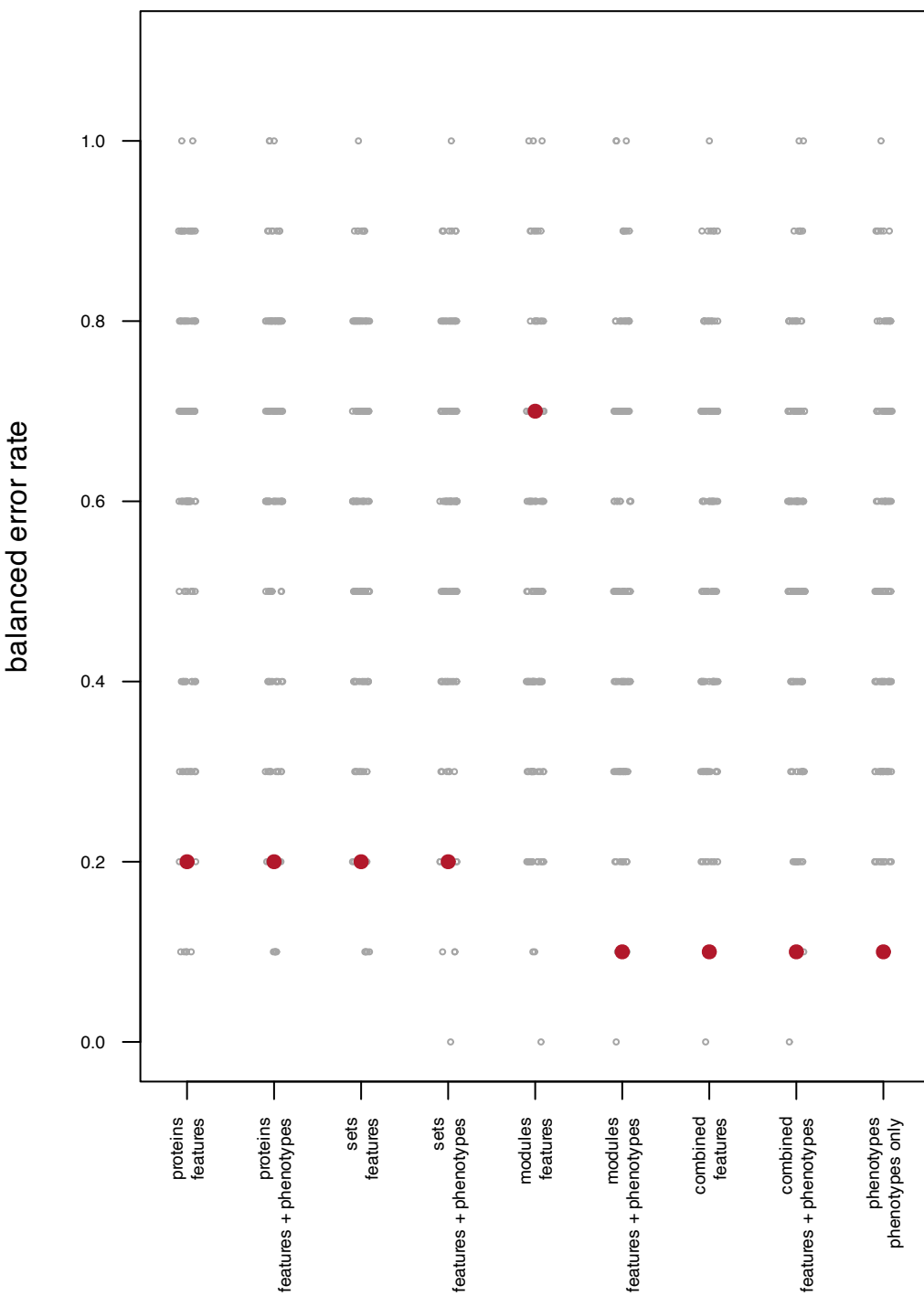
PAS_vs_VEH_female: DIABLO / sPLS-DA
