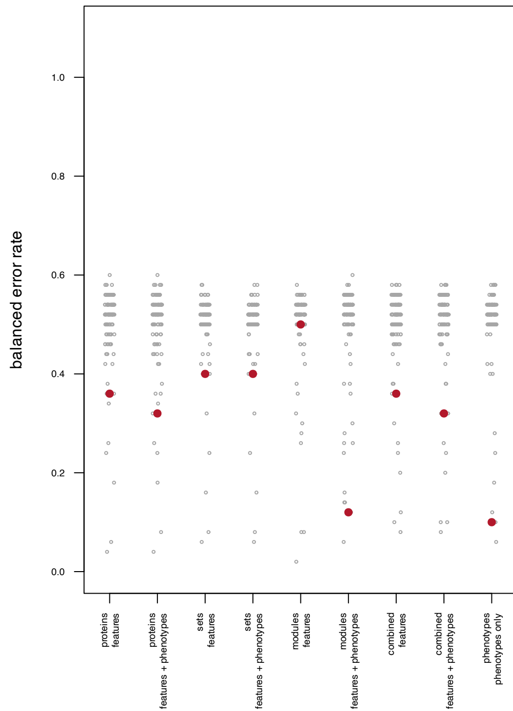
PAS_vs_VEH_female: elastic net (nestedcv)
