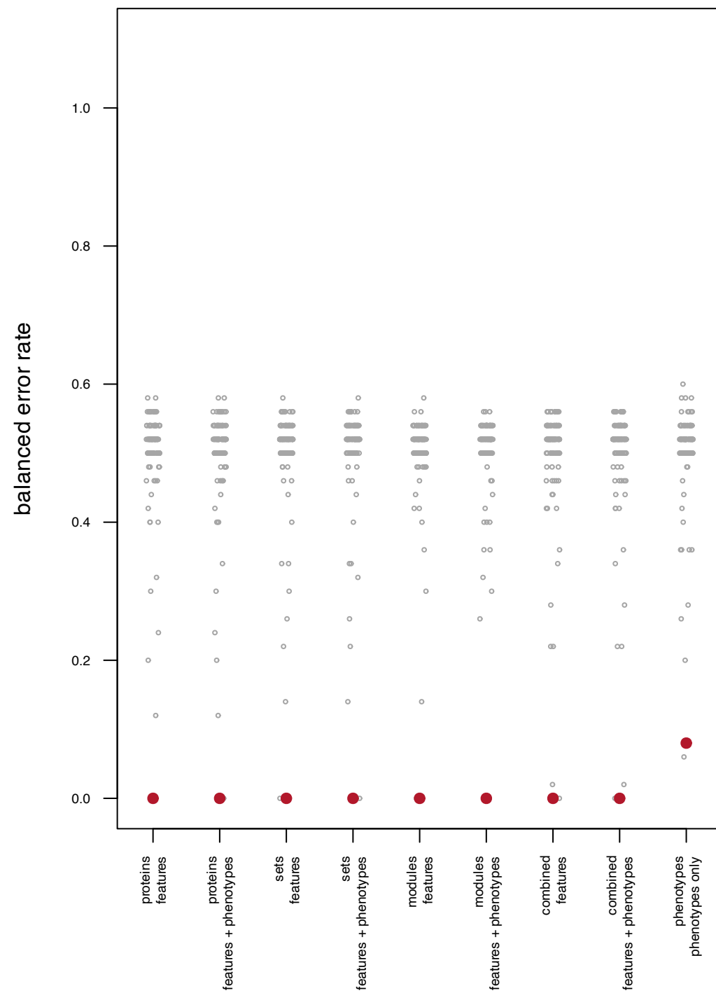
sex_in_VEH: elastic net (nestedcv)
