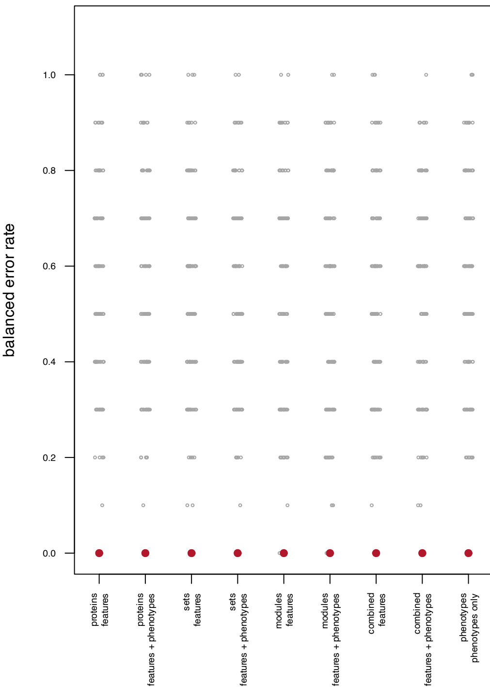
sex_in_VEH: DIABLO / sPLS-DA
