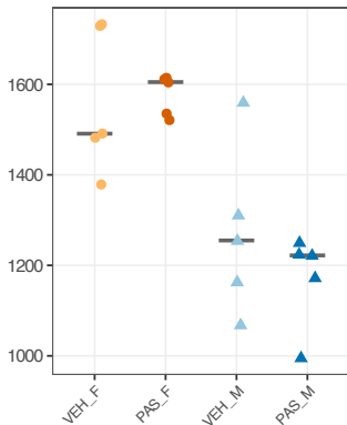
Protein groups
