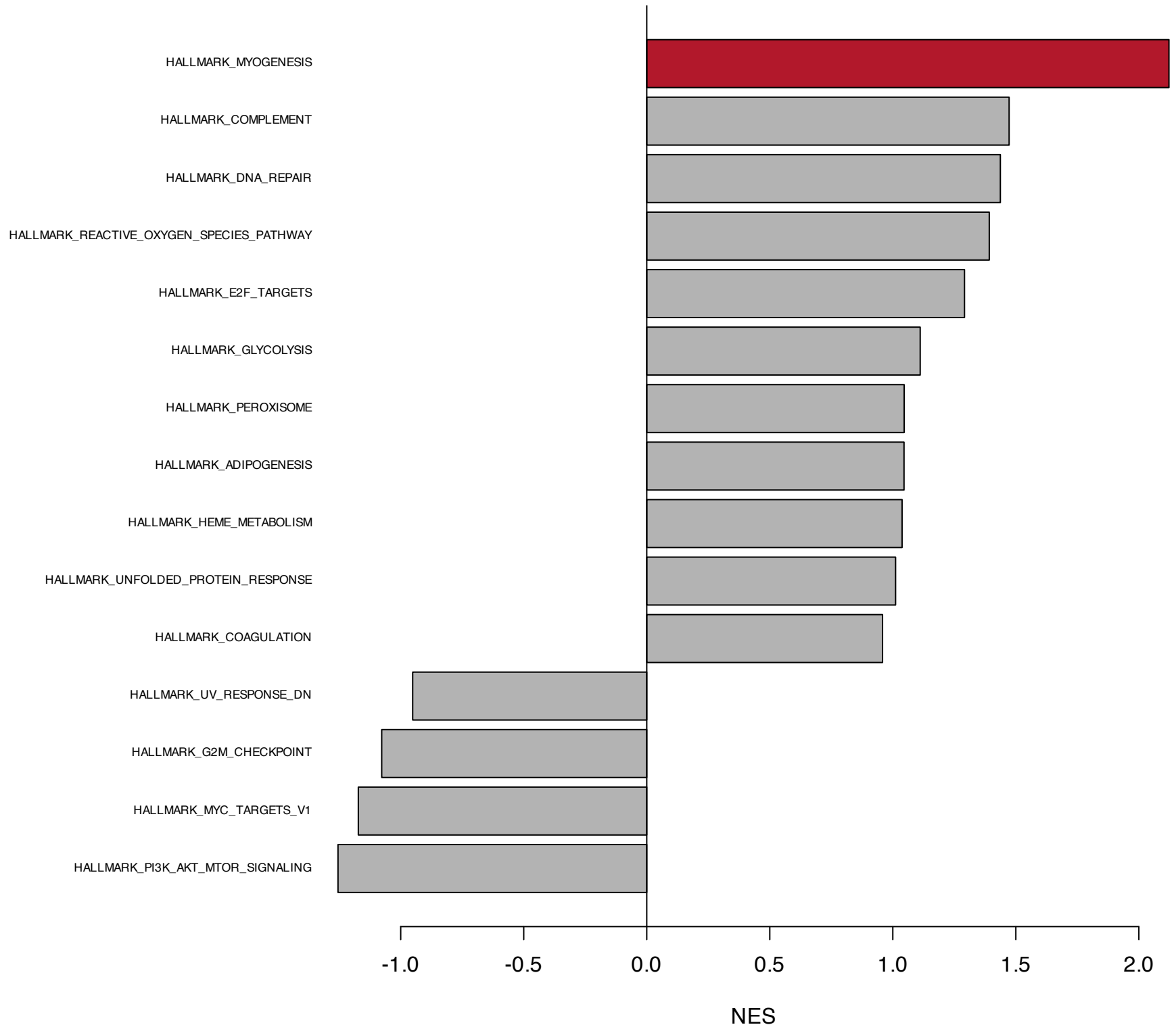
PAS_vs_VEH_female: Hallmark, 15 smallest p (red: FDR \leq 0.05)
