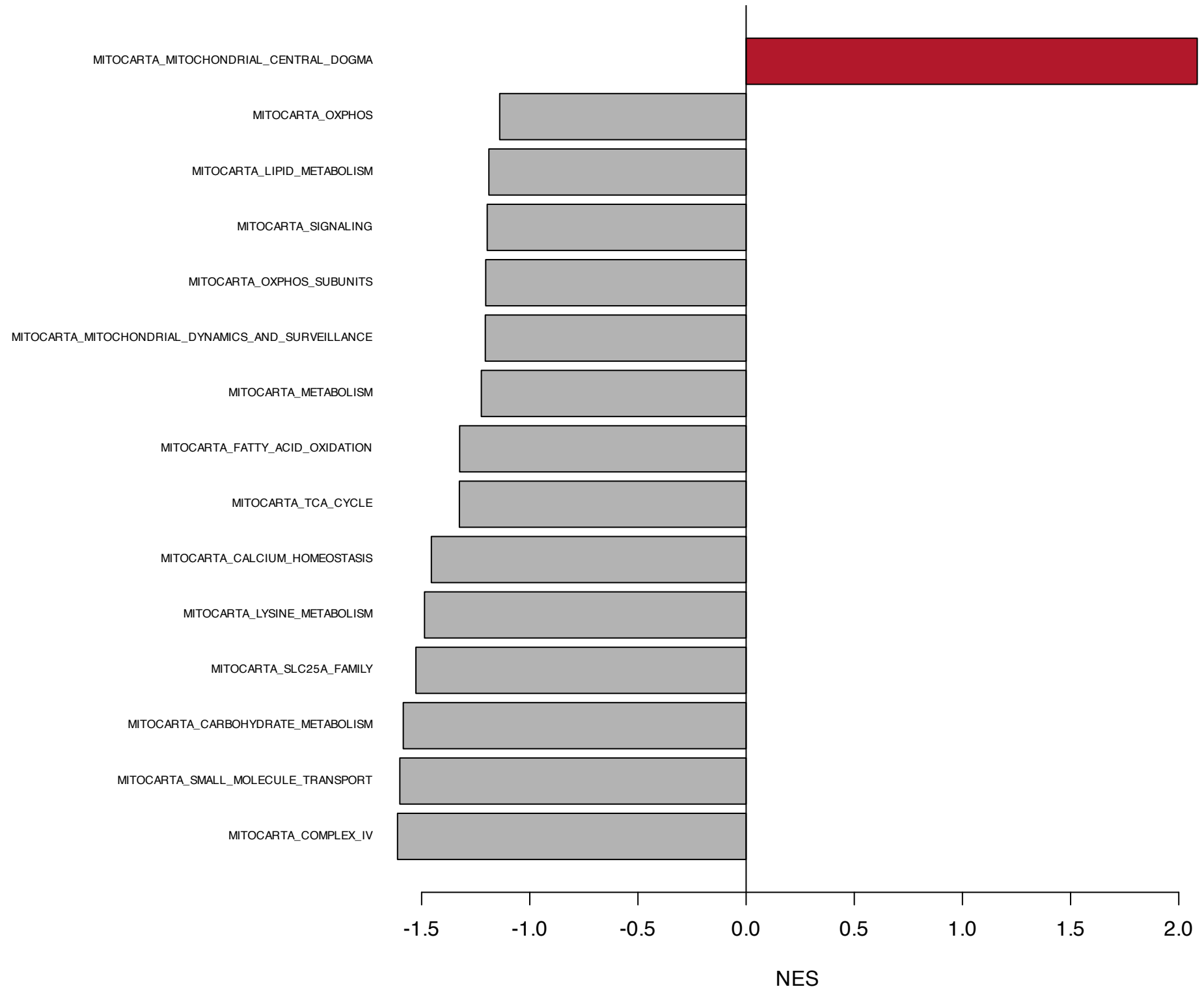
PAS_vs_VEH_male: MitoCarta, 15 smallest p (red: FDR \leq 0.05)
