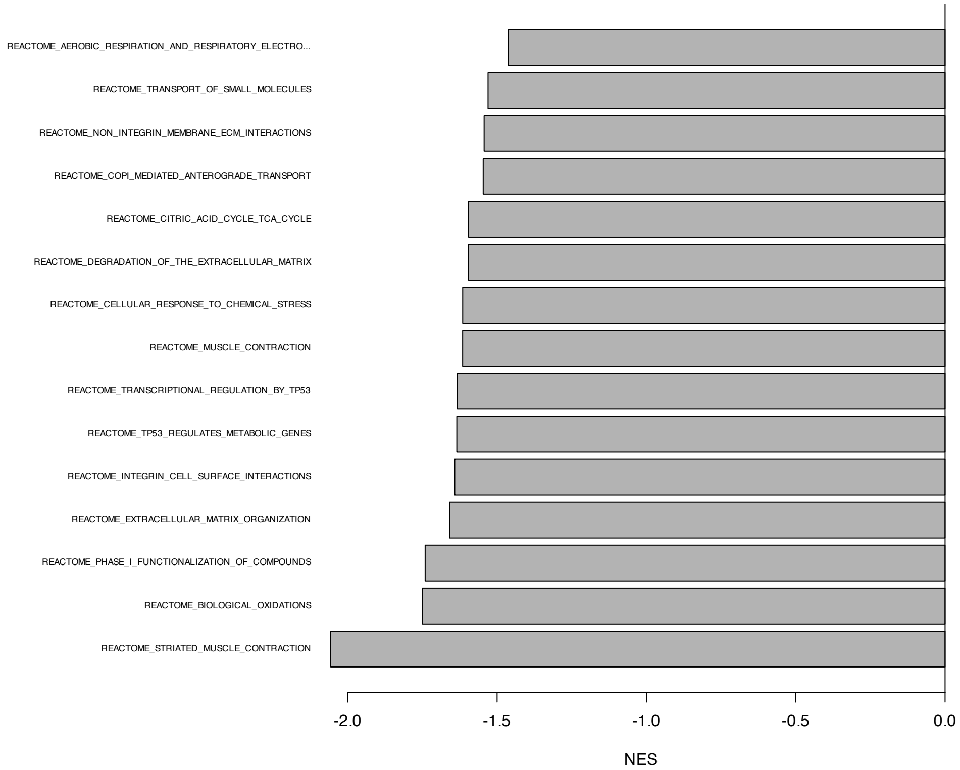
PAS_vs_VEH_male: Reactome, 15 smallest p (red: FDR \leq 0.05)
