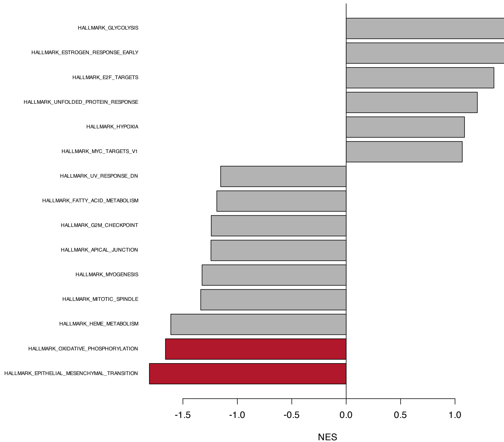
PAS_vs_VEH_male: Hallmark, 15 smallest p (red: FDR ≤ 0.05)
