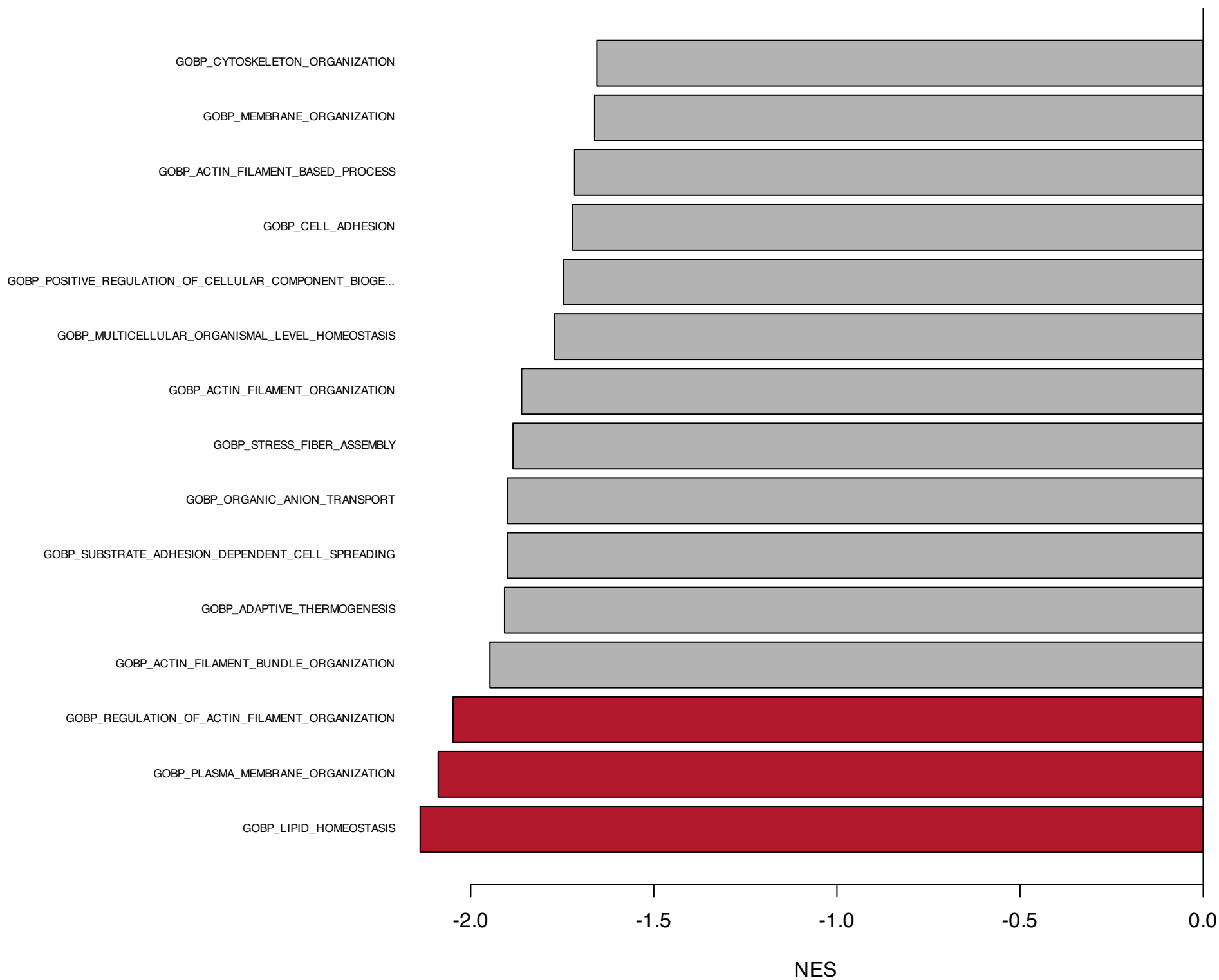
PAS_vs_VEH_male: GO:BP, 15 smallest p (red: FDR ≤ 0.05)
