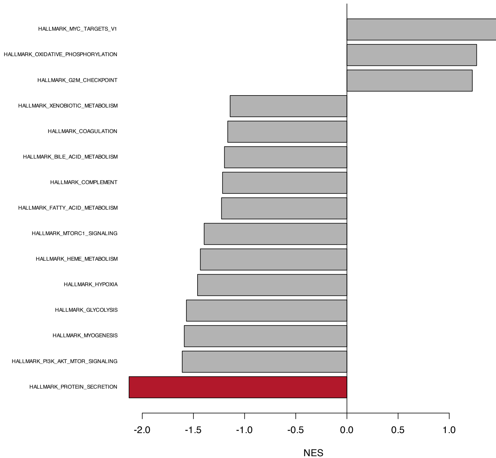
sex_in_PAS: Hallmark, 15 smallest p (red: FDR ≤ 0.05)
