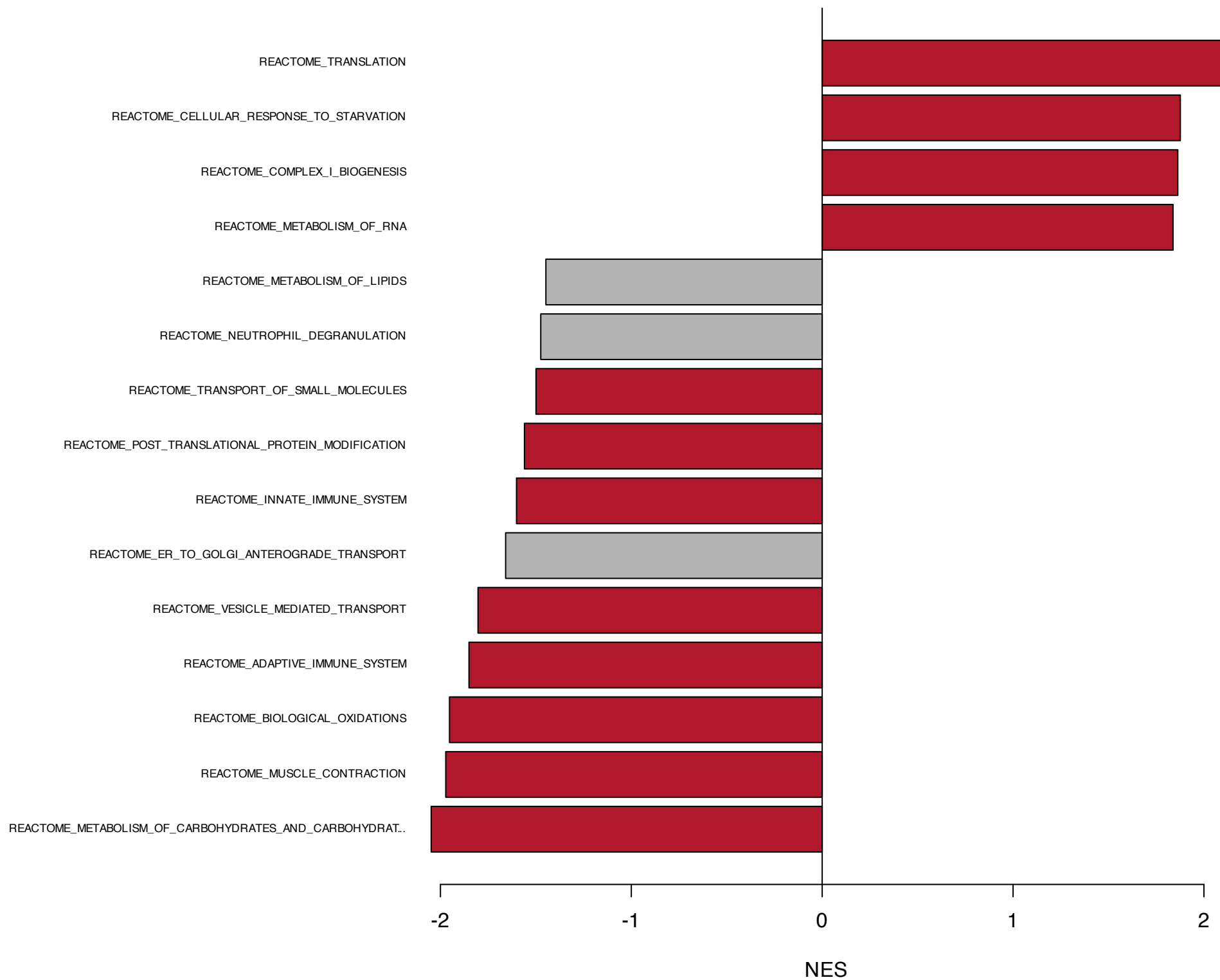
sex_in_PAS: Reactome, 15 smallest p (red: FDR ≤ 0.05)
