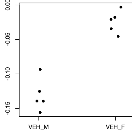
REACTOME_CLASS_II_MHC_MEDIATED_ANTIGEN_PRESENTATION AUC 0.00, p 0.008
