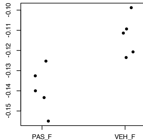
GOBP_REGULATION_OF_CELL_CYCLE AUC 0.00, p 0.008
