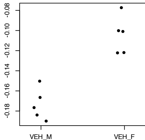
REACTOME_CELL_CYCLE AUC 0.00, p 0.008
