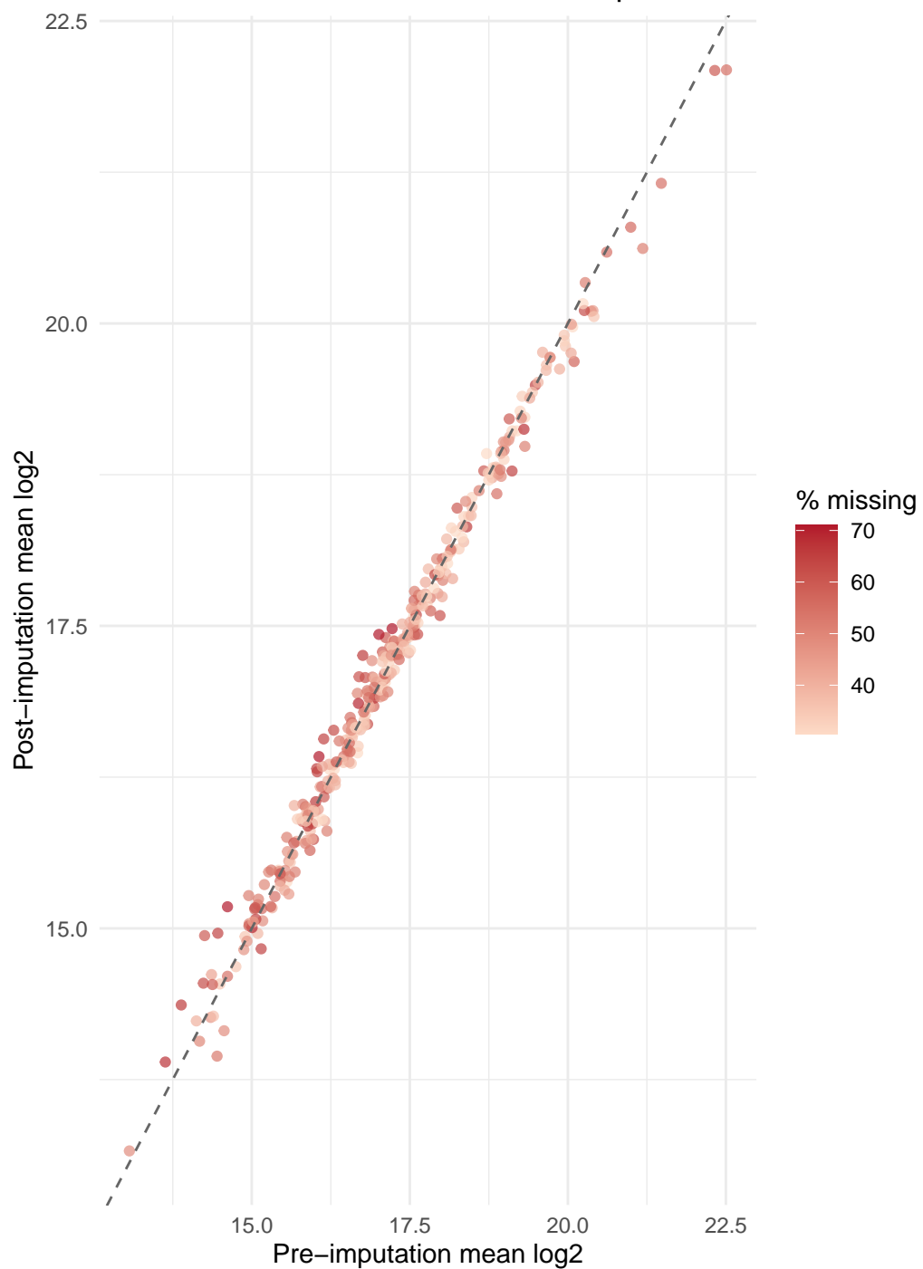
A: MNAR Protein Mean Shift After Imputation
