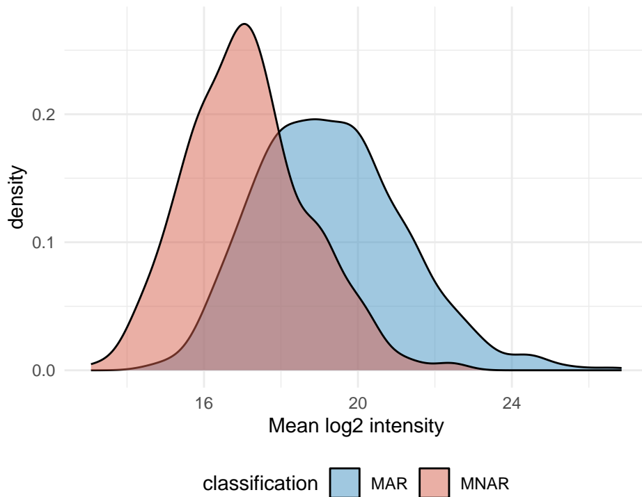
B: Intensity by Missingness Type
