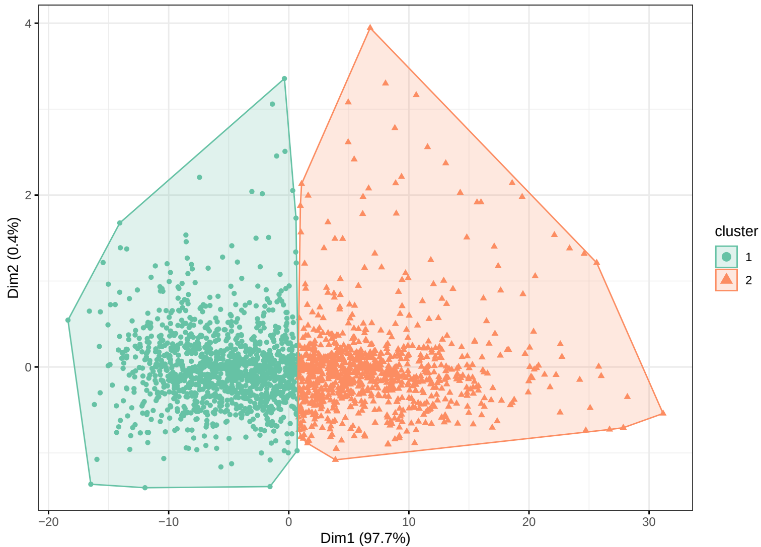
K-means clustering (k=2, Imputed)
