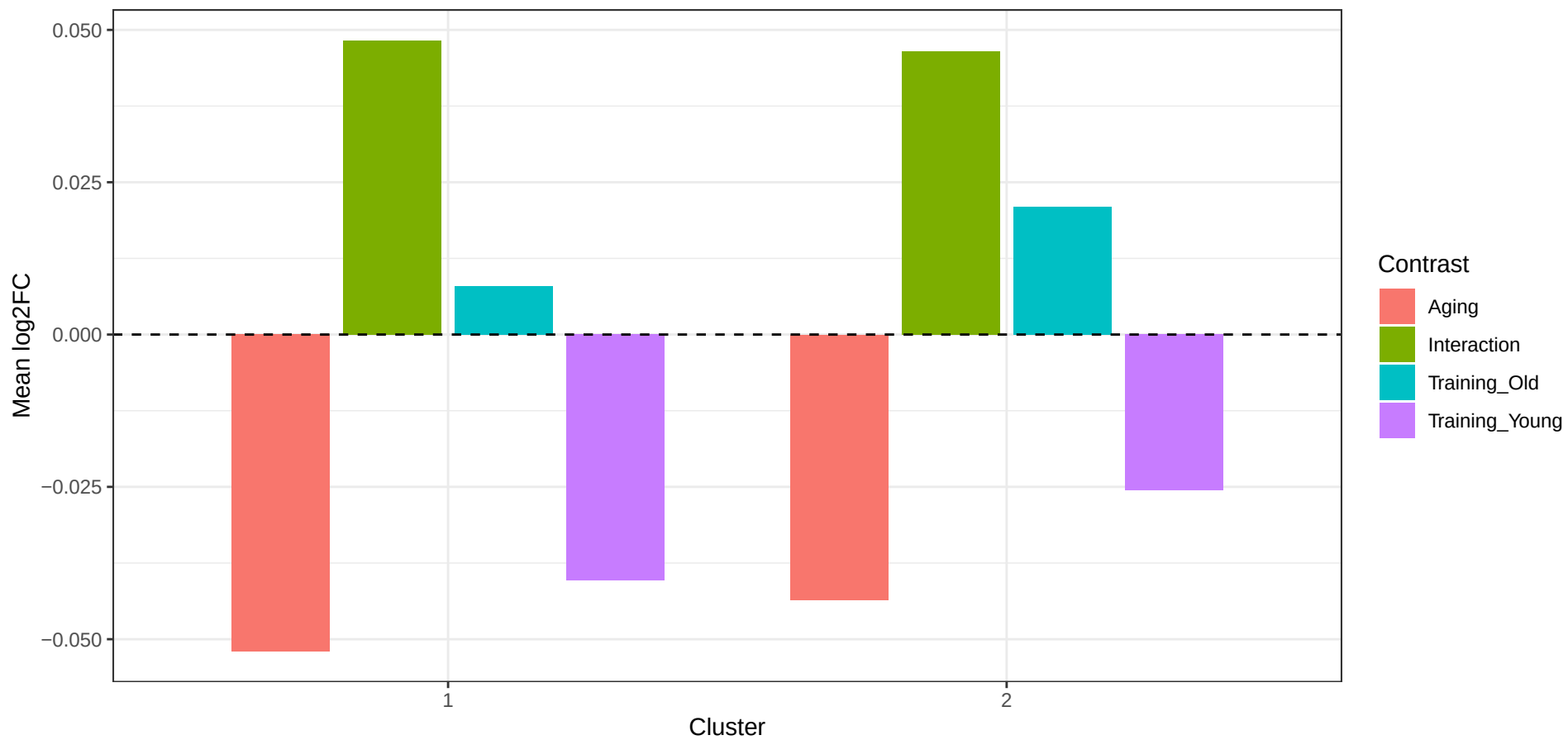
Cluster characterization by DEP logFC (Imputed)
