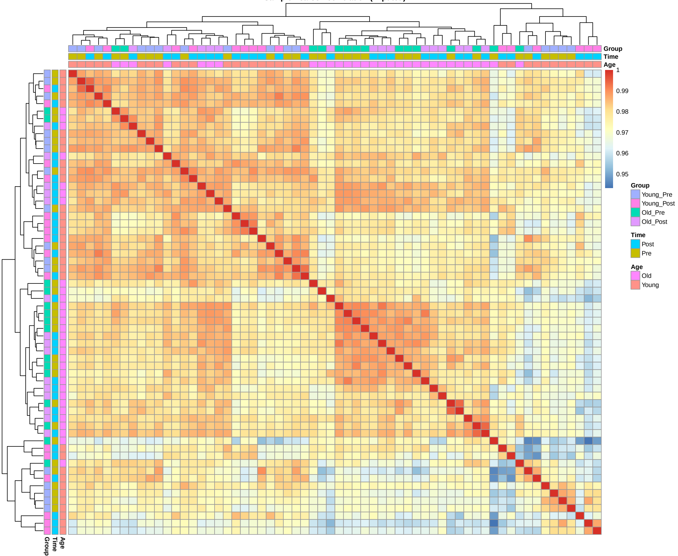
Sample Pearson correlation (Imputed)
