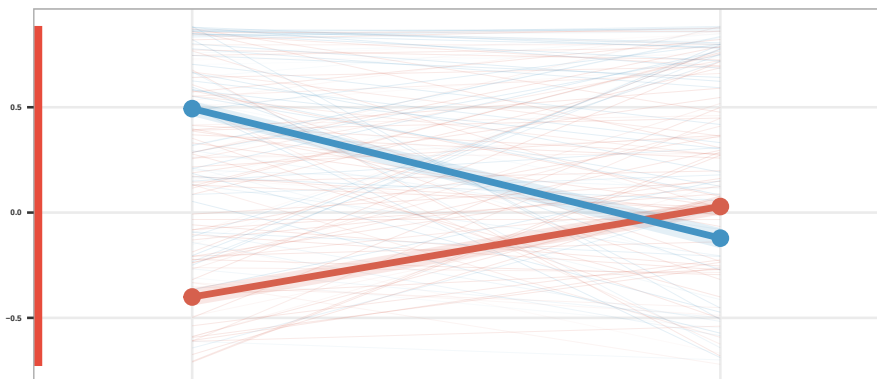
C2: mTORC1 Signaling (n = 563)
