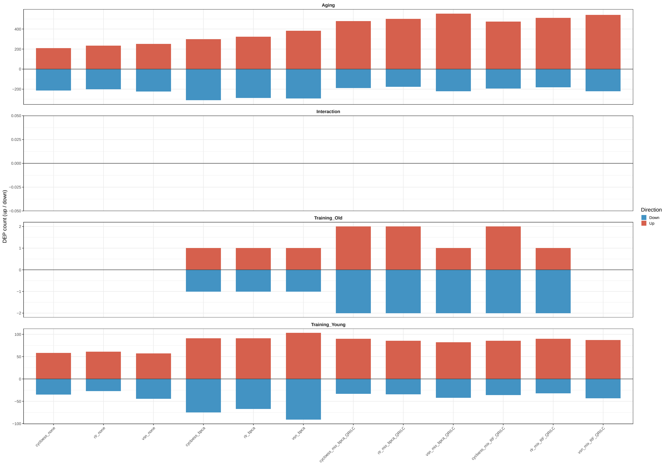
DEP counts per pipeline (FDR &lt; 0.05)
