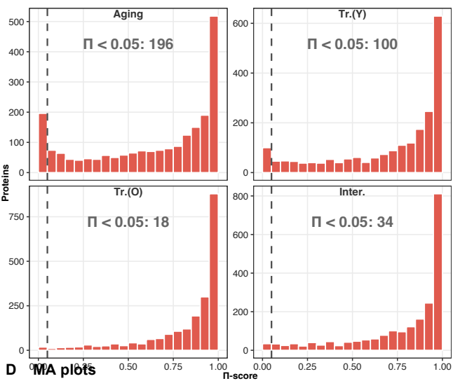
B \Pi -score distribution
