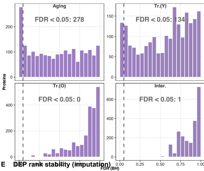
C FDR distribution
