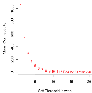
Mean connectivity
