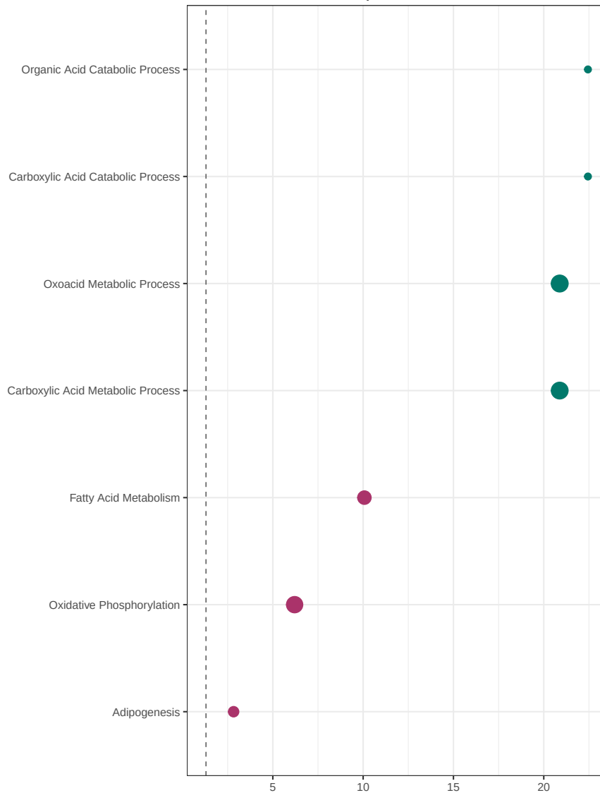
Blue – Lipid/AA Catabolism
