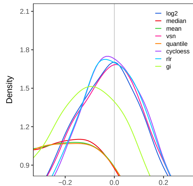
Log2 ratio
