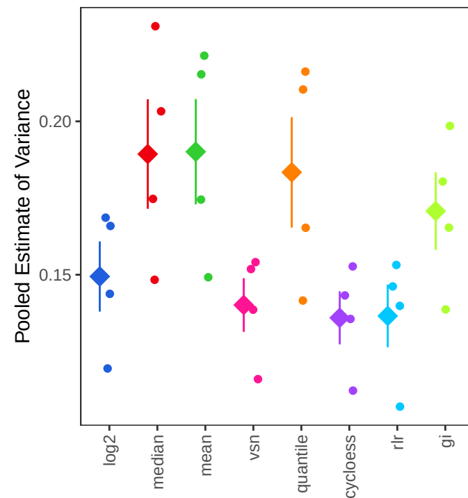
Log2 ratio
