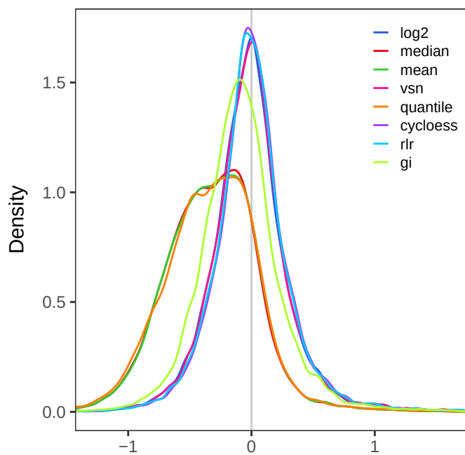
Log2 ratio
