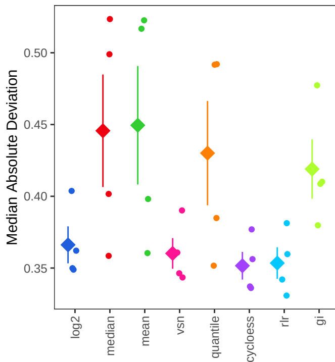
Log2 ratio
