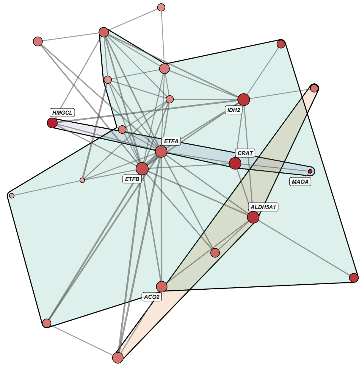
M4: Redox/Glycolysis 17 nodes | Node color: GS (Age (Younger), Older)
