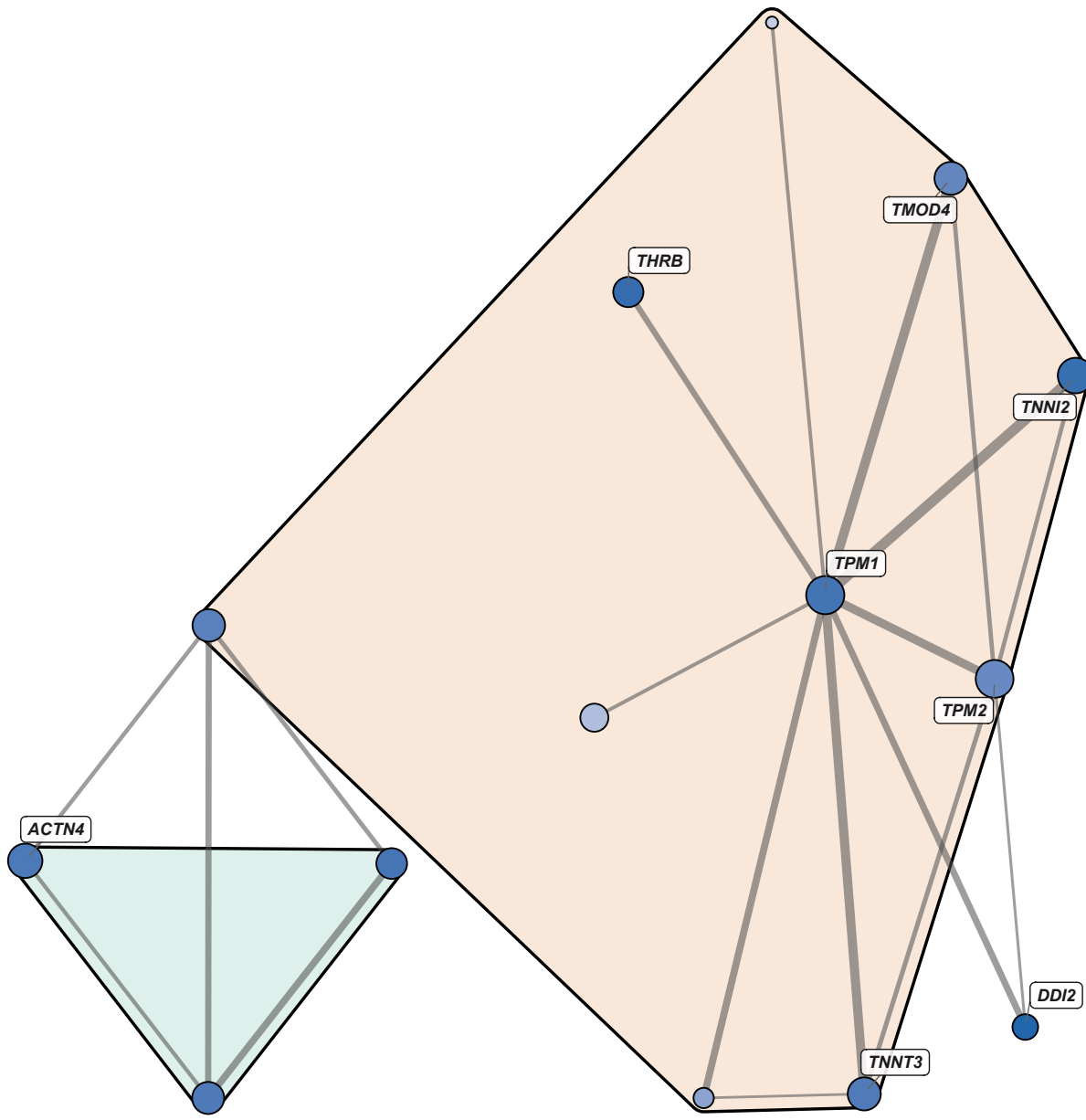
M6: Immunity/Immune 15 nodes | Node color: GS (Age (Younger), Older)
