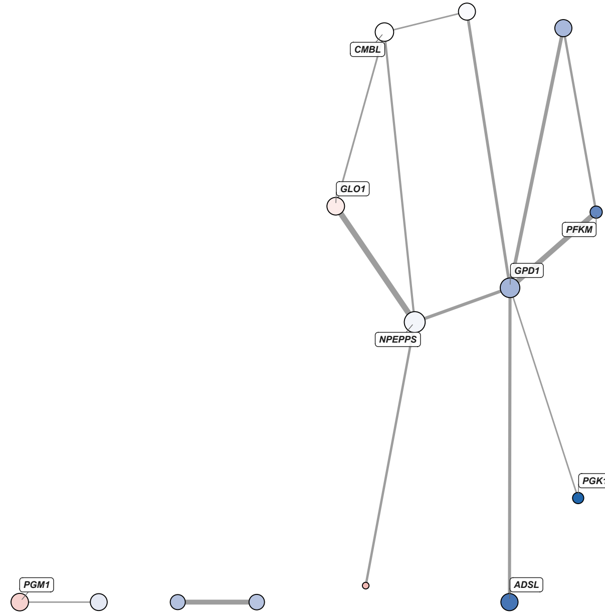
M7: Translation Machinery 13 nodes | Node color: GS (Age (Younger), Older)
