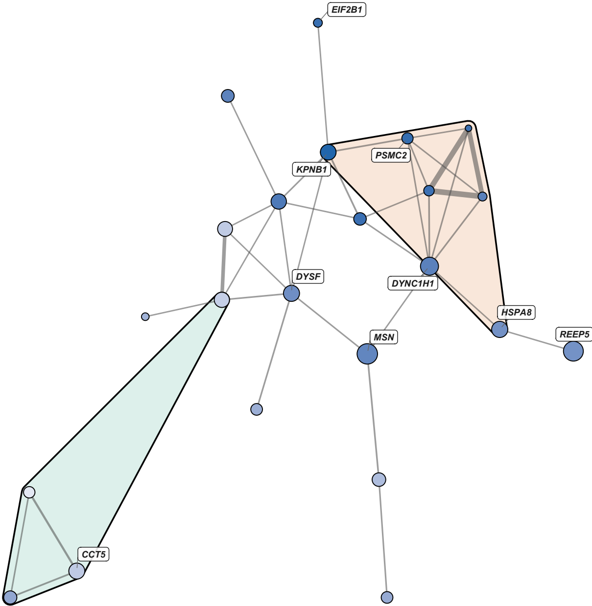
M2: Cell Cycle / Proteostasis (Chaperones) 27 nodes | Node color: GS (Age (Young=0, Old=1))
