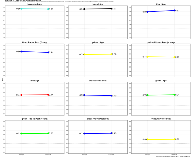
D. Top layer - Full WGCNA with L000 sensitivity
