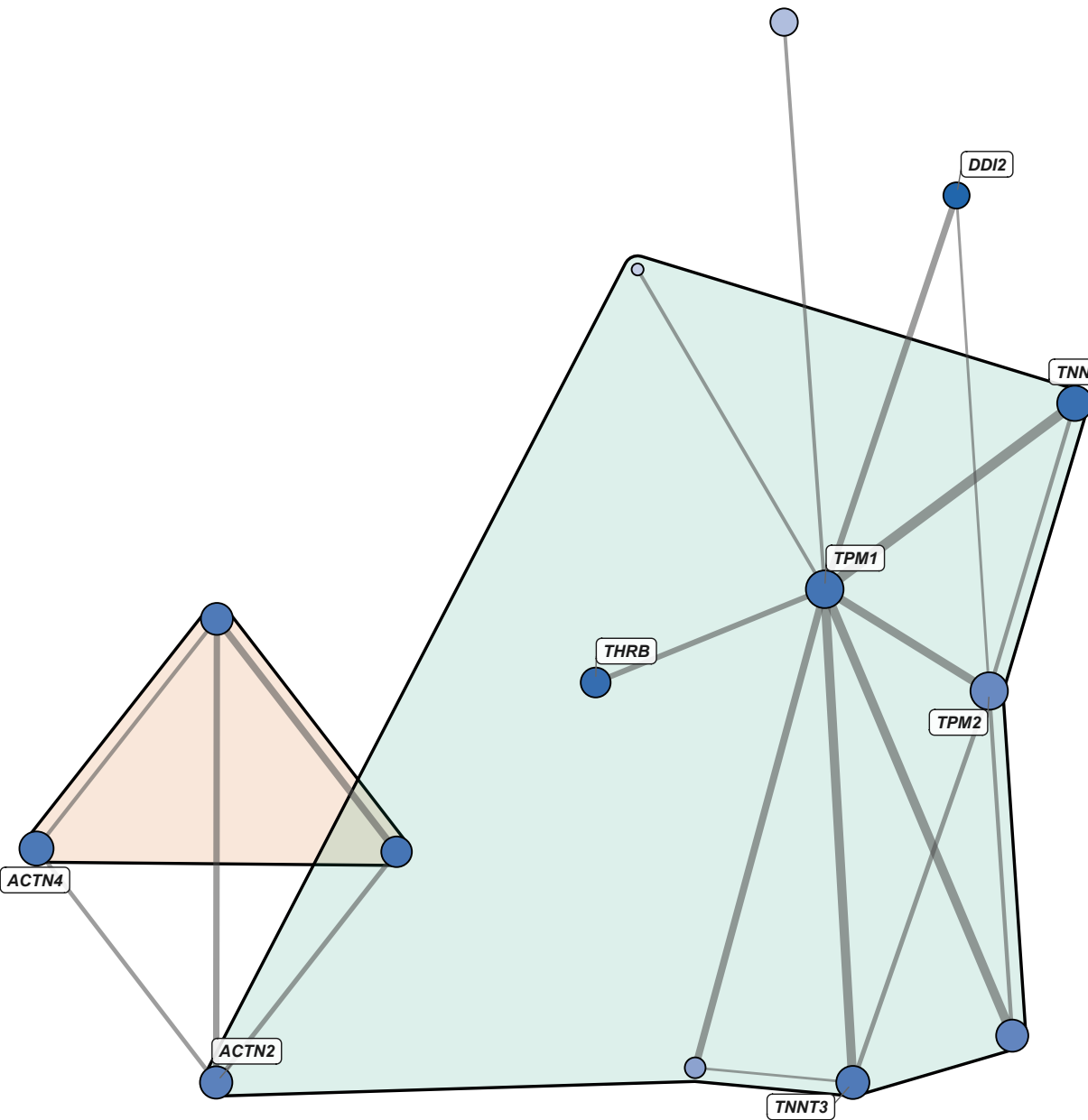
M7: UPS 9 nodes | Node color: GS (Age (Young=0, Old=1))
