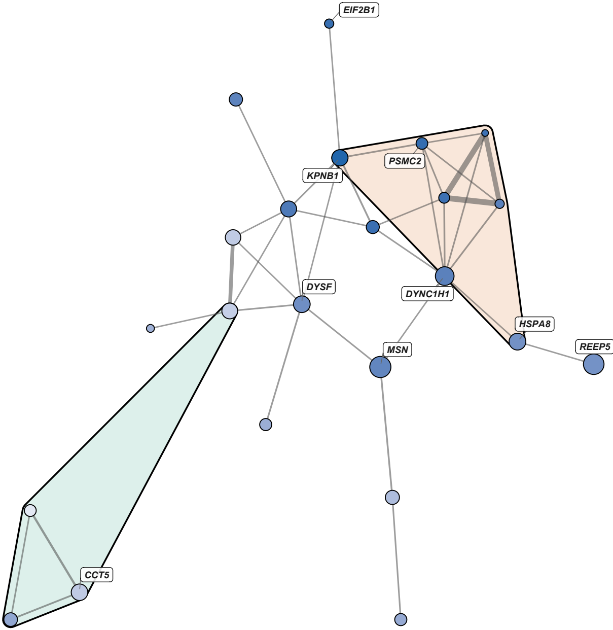
M2: Cell Cycle/Proteostasis 27 nodes | Node color: GS (Age (Young=0, Old=1))
