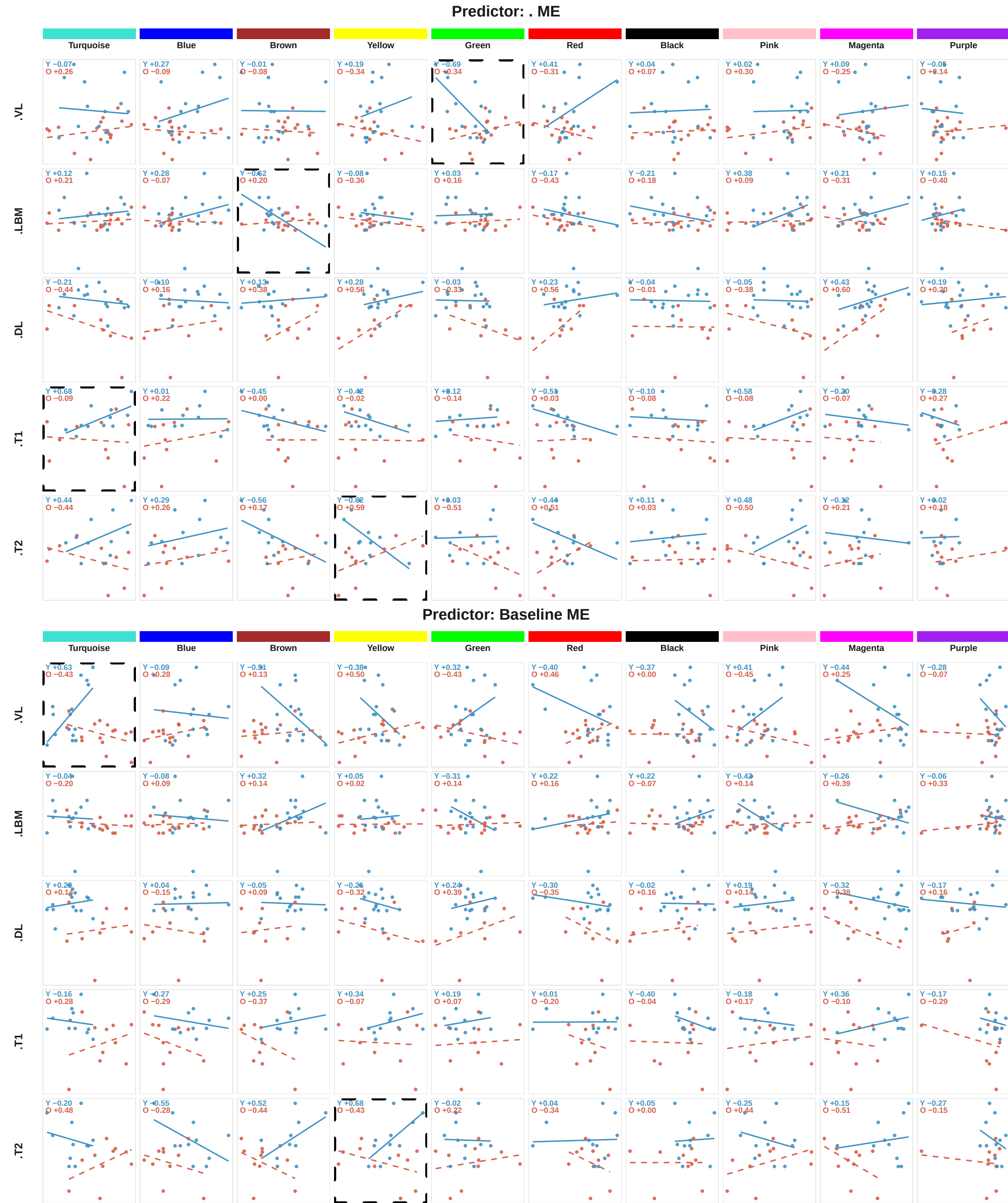
F07 SUPP – Panel B full sweep: module eigengenes vs .phenotype, age-stratified Border emphasis: thick solid black = BH q<0.05; thick dashed = nominal p<0.05 in Young; thin grey = ns. Lines = per-age OLS (Young solid, Old dashed). Screen: 200 tests (2 sources × 10 modules × 5 outcomes).
