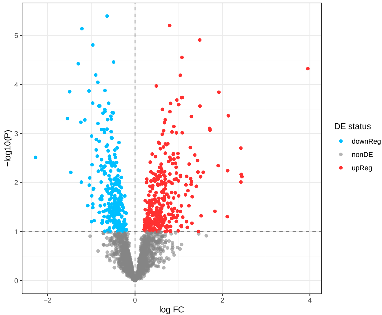
Reversal, raw p-value
