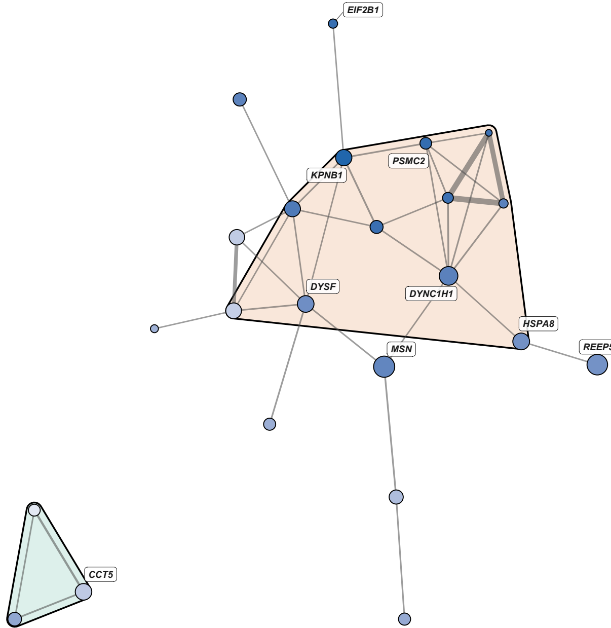
M2: Cell Cycle / Proteostasis (Chaperones) 27 nodes | Node color: GS (Age (Young=0, Old=1))
