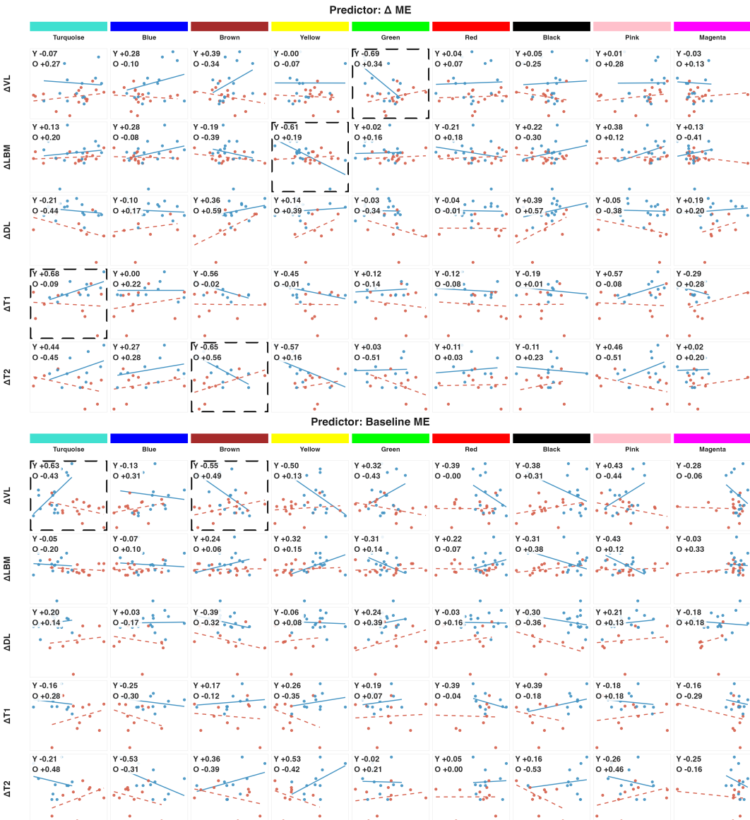
B F07 Supplementary — Panel B full sweep: module eigengenes vs Δ phenotype, age-stratified
