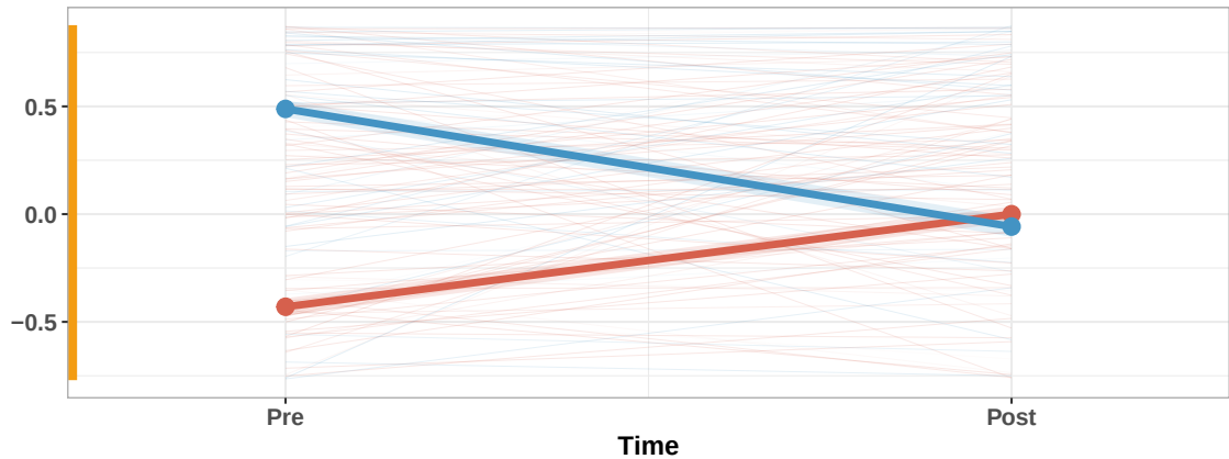
C4: Myogenesis (n = 386)
