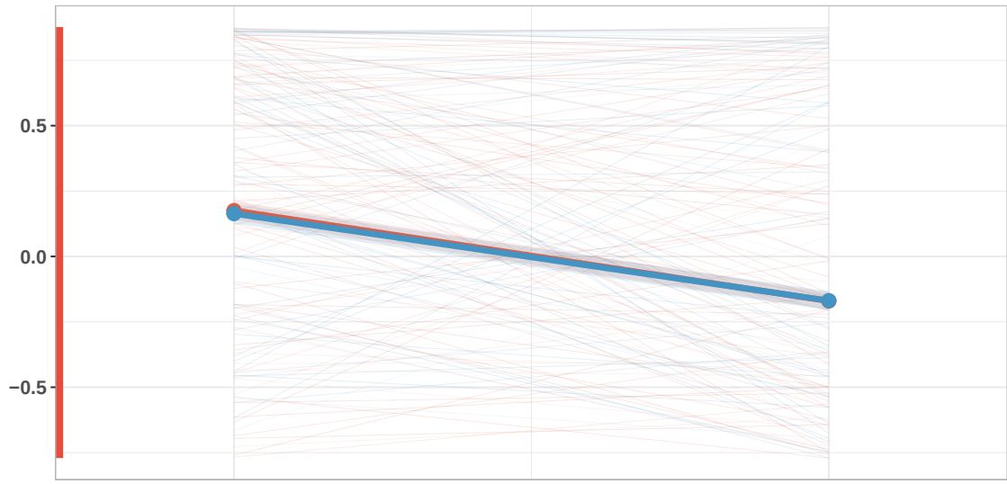
C2: Oxidative Phosphorylation (n = 537)
