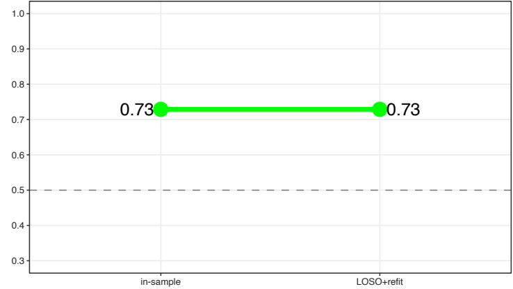
green | Pre vs Post (Young)
