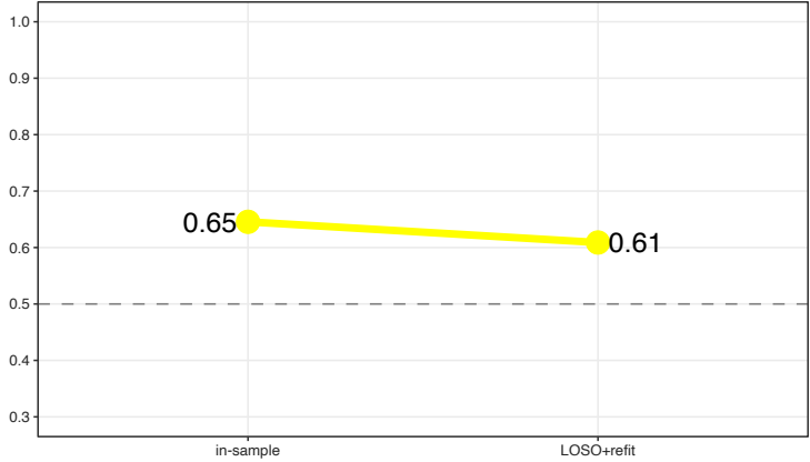
yellow | Pre vs Post
