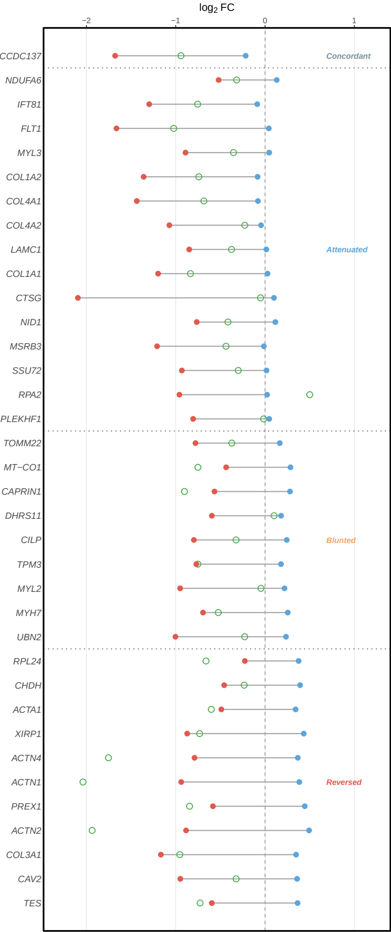
Interaction DEPs: Multi-Contrast Response & Pathway Enrichment 36 proteins with significant Age x Training interaction ( p_i < 0.05 )
