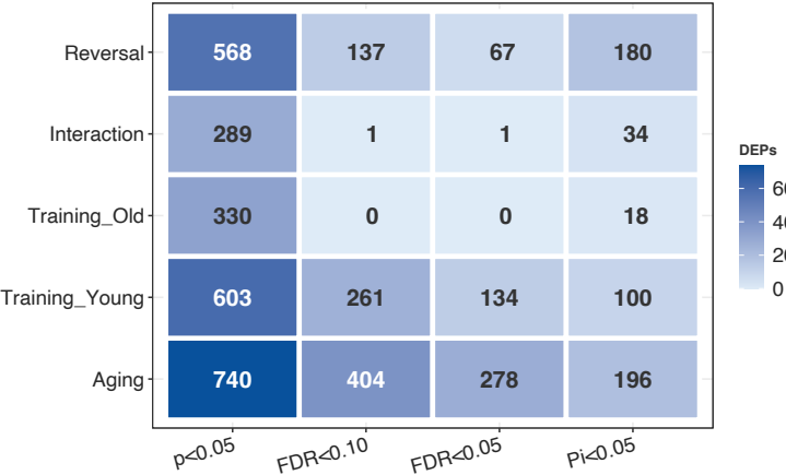
DEP counts: contrast x threshold
