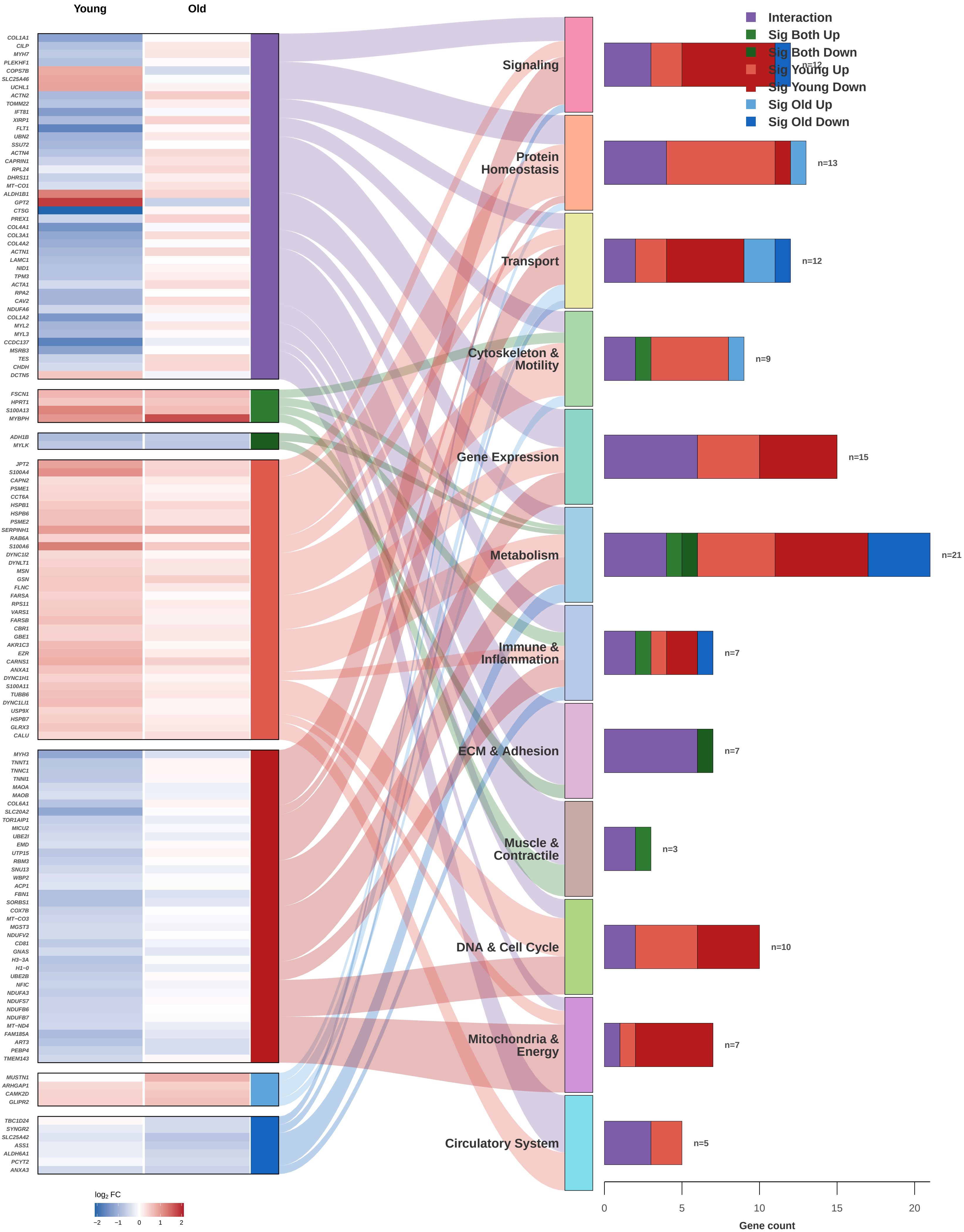
Significant Proteins: Multi-Category Heatmap & Pathway Enrichment 131 proteins across 7 significance categories | GO Slim super-categories (Fisher, BH adj.)
