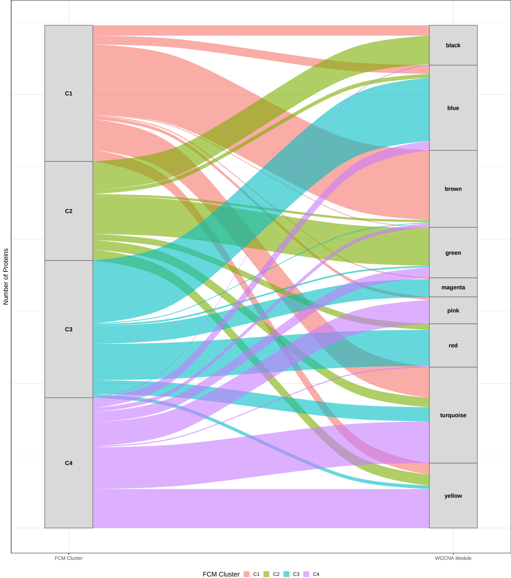
FCM Temporal Cluster – WGCNA Module Overlap 1743 proteins | ribbons show shared membership | 32 significant pairs (BH < 0.05)
