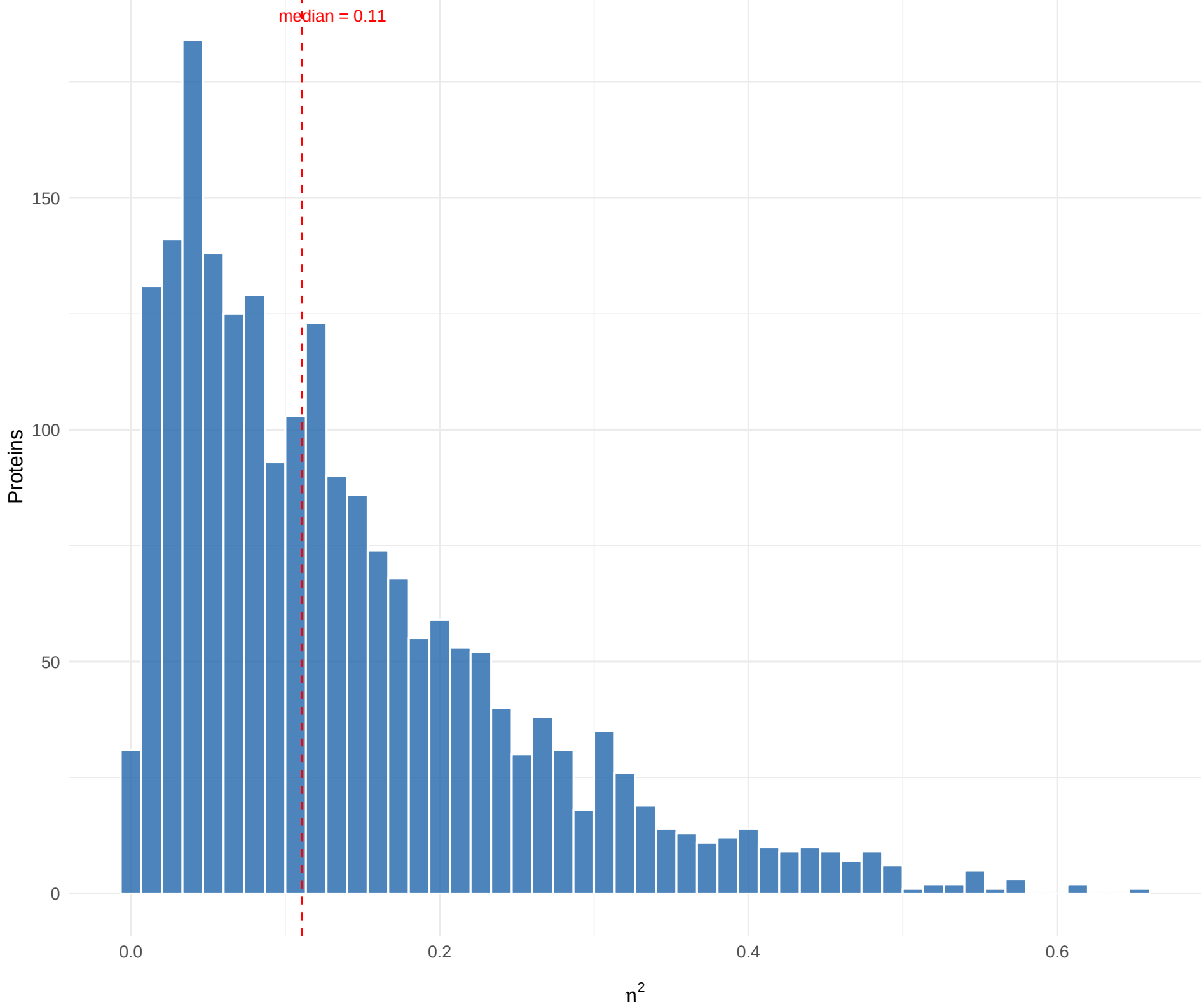
Variance partition by group
