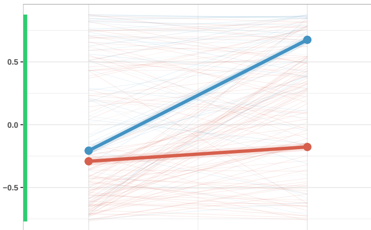
Cluster 4 ( n = 386 )
