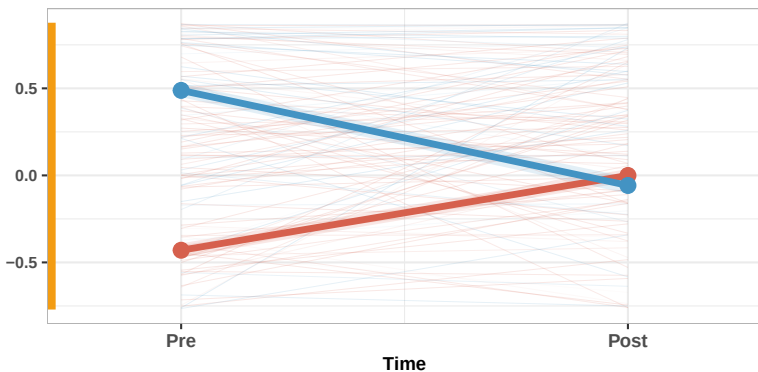
Cluster 4 ( n = 386 )
