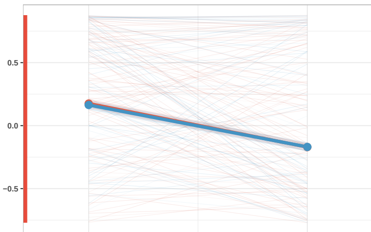
Cluster 2 ( n = 537 )
