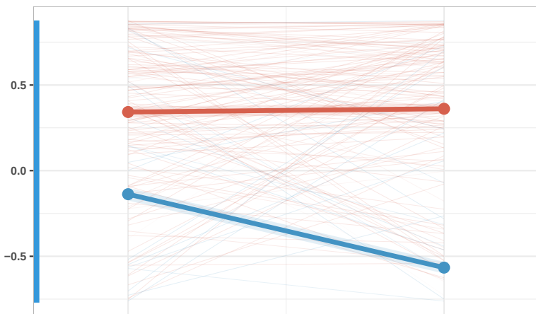
Cluster 3 ( n = 569 )
