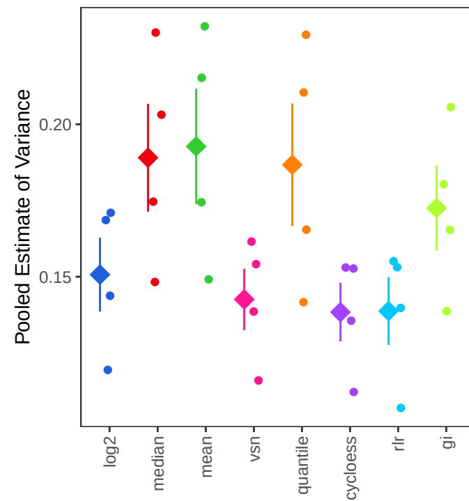
Log2 ratio
