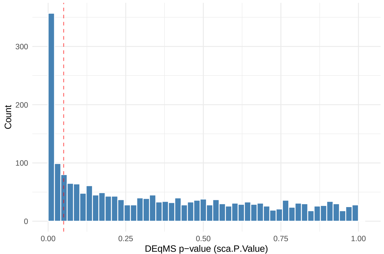
Training_Young – P-value Distribution (DEqMS)
