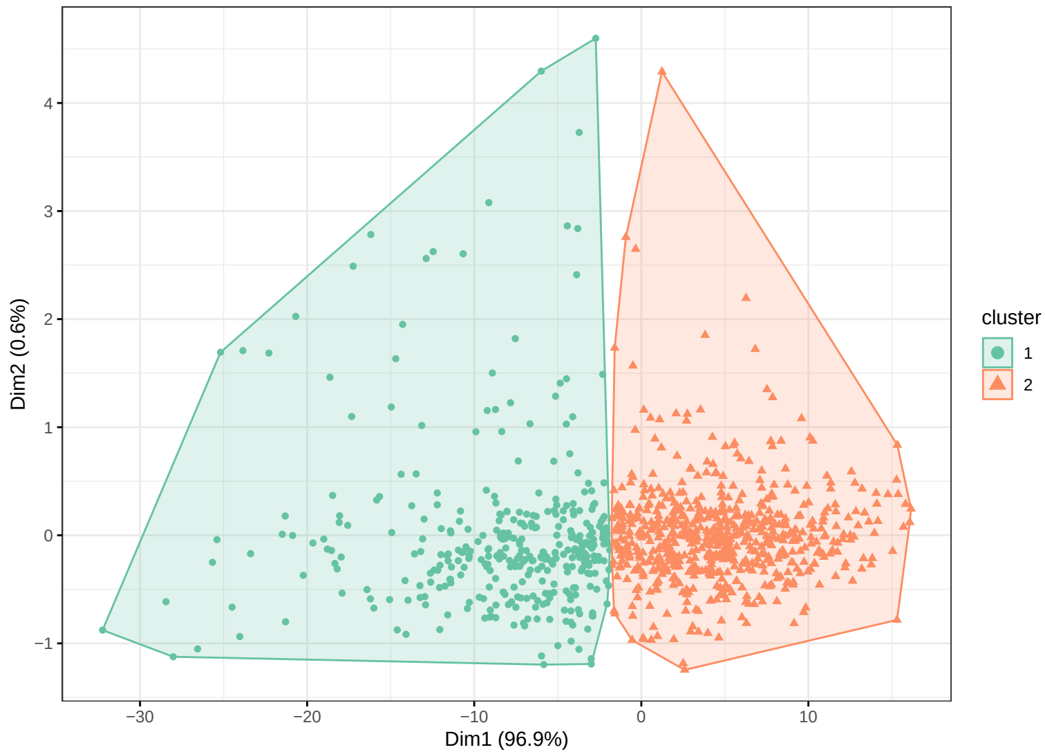
K-means clustering (k=2, Non-imputed, 987 proteins)
