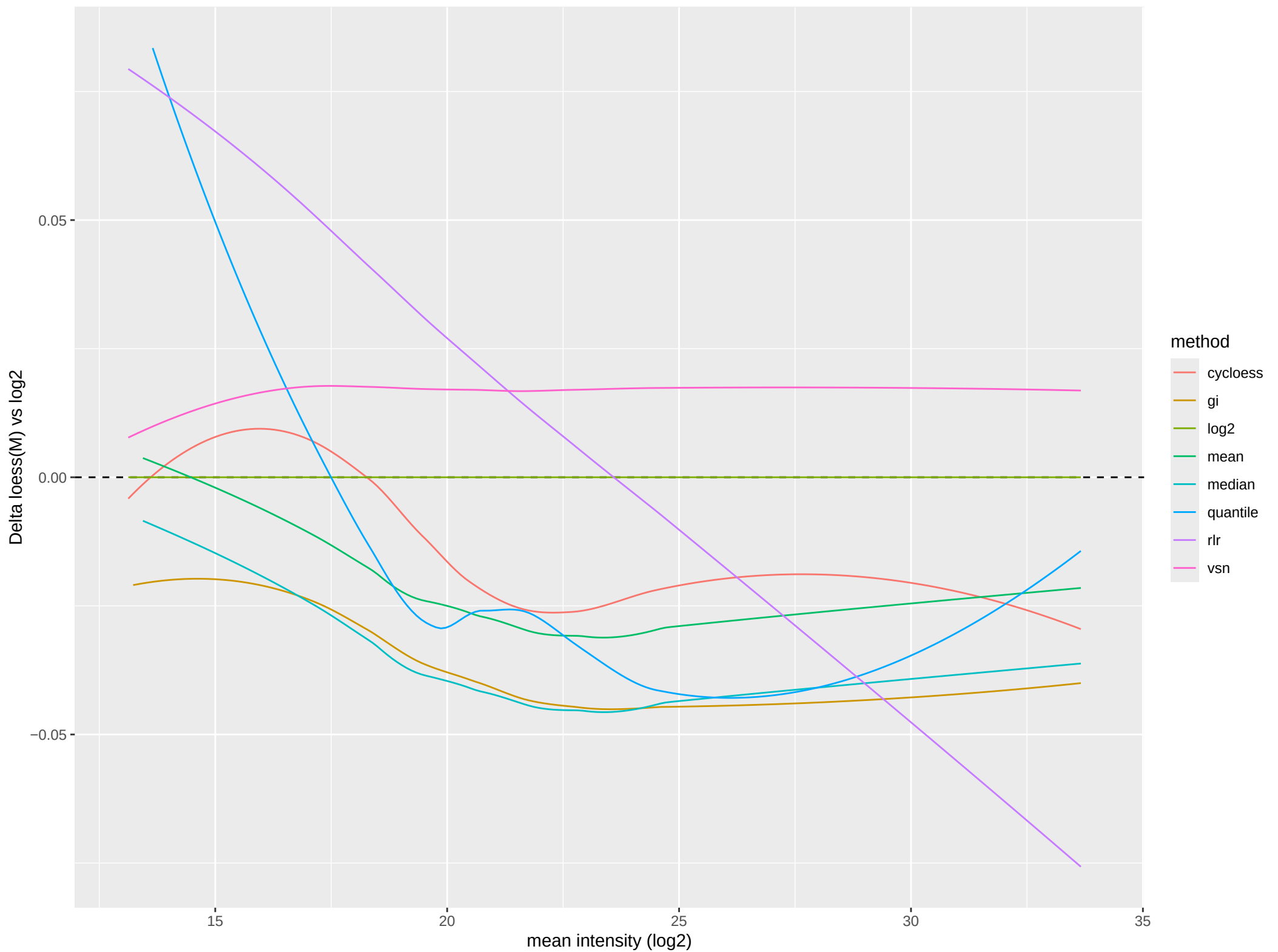
Delta-trend vs raw log2 (over-/under-correction) – GLOBAL
