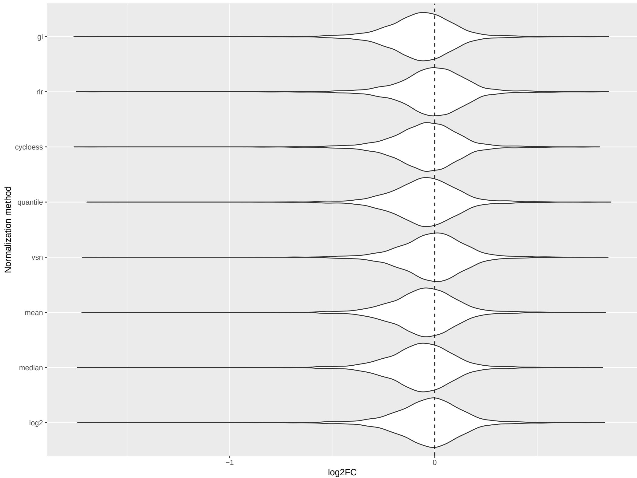
log2FC distributions by normalization – GLOBAL
