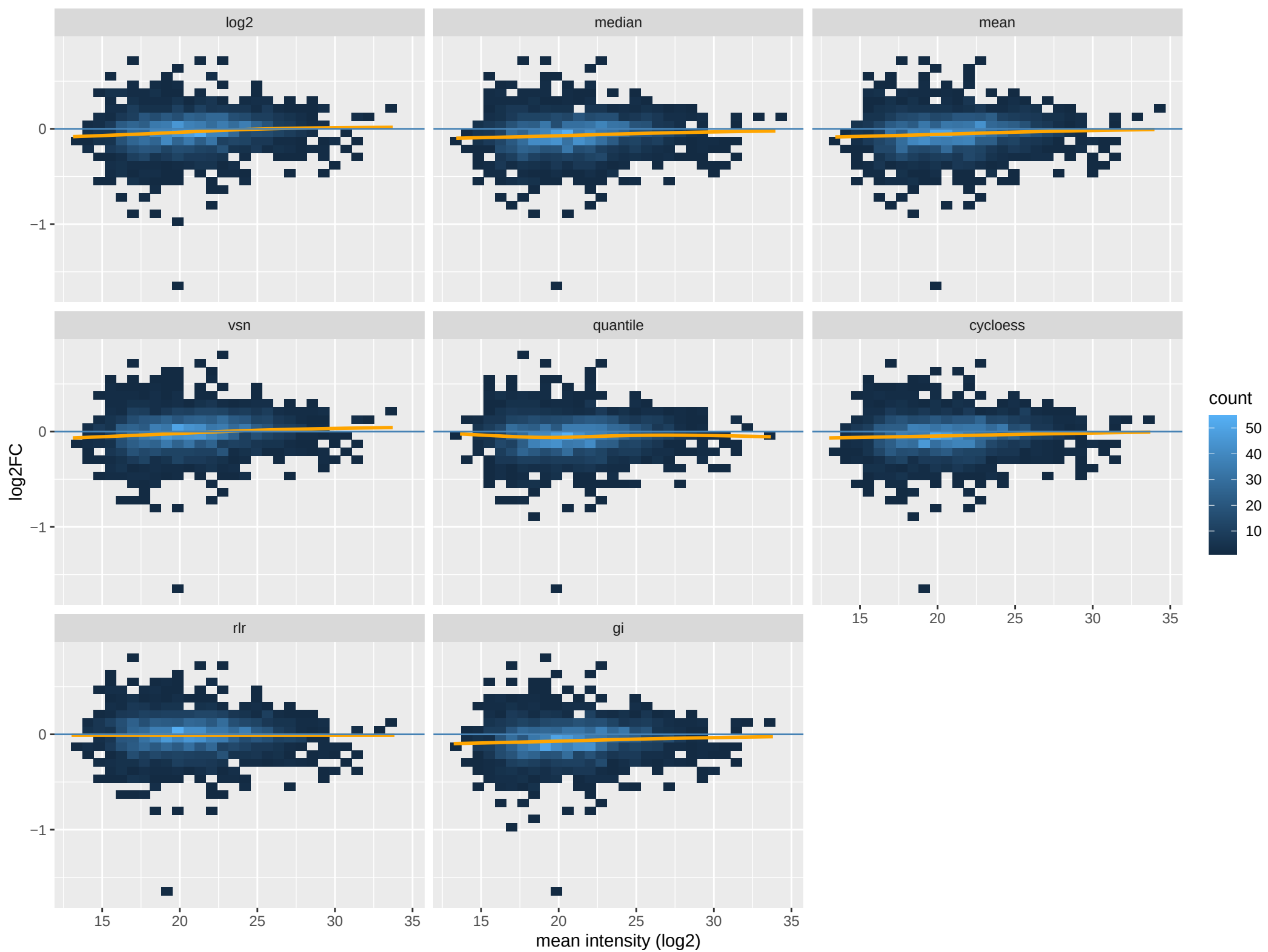
MD plots (2D-binned density + trend) – GLOBAL
