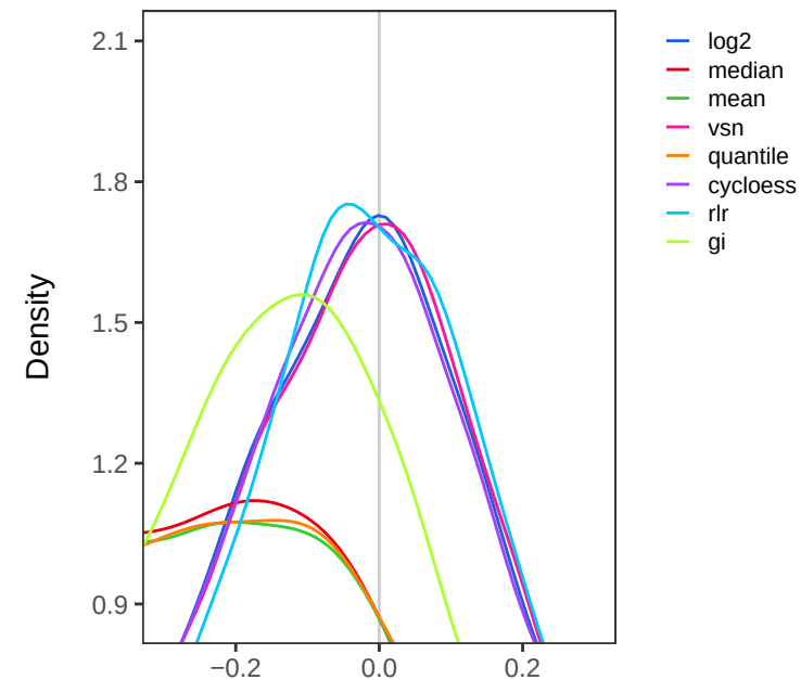
Log2 ratio
