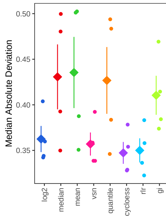
Log2 ratio
