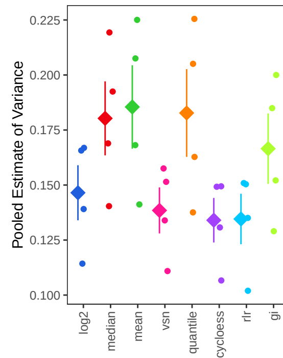
Log2 ratio
