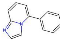
5-Phenylimidazo[1,2-a]pyridine
