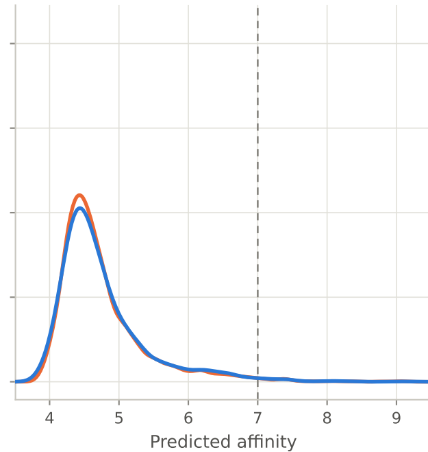
ZeroGEN
