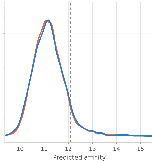
ZeroGEN
